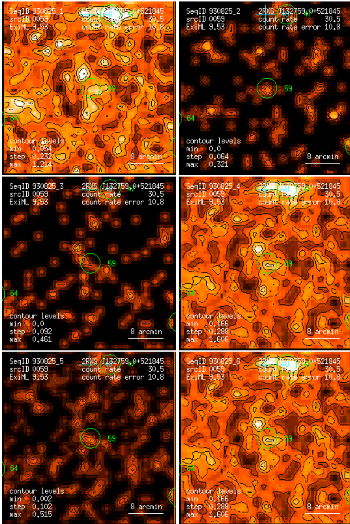
Figure 59: RASS 930825: detection 0059: band rate images, Gaussian filter: (1) PSPC channels 11 – 41, (2) 52 – 90, (3) 91 – 201, (4) 11 – 235, (5) 52 – 201, (6) 11 – 201. Broad band rates in counts/ks. Band rate contour levels in counts/ks/arcmin 2 .
