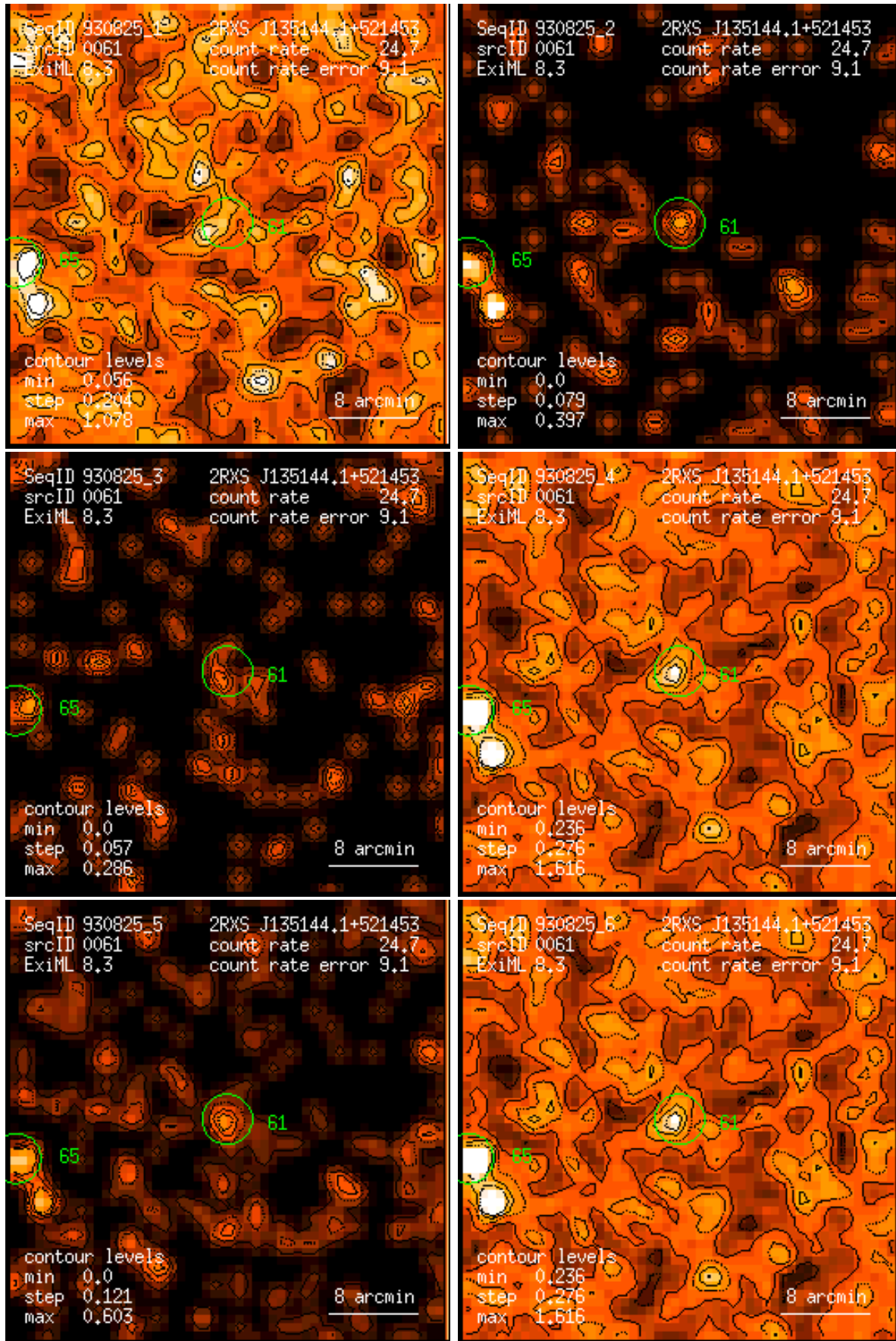
Figure 61: RASS 930825: detection 0061: band rate images, Gaussian filter: (1) PSPC channels 11 – 41, (2) 52 – 90, (3) 91 – 201, (4) 11 – 235, (5) 52 – 201, (6) 11 – 201. Broad band rates in counts/ks. Band rate contour levels in counts/ks/arcmin 2 .
