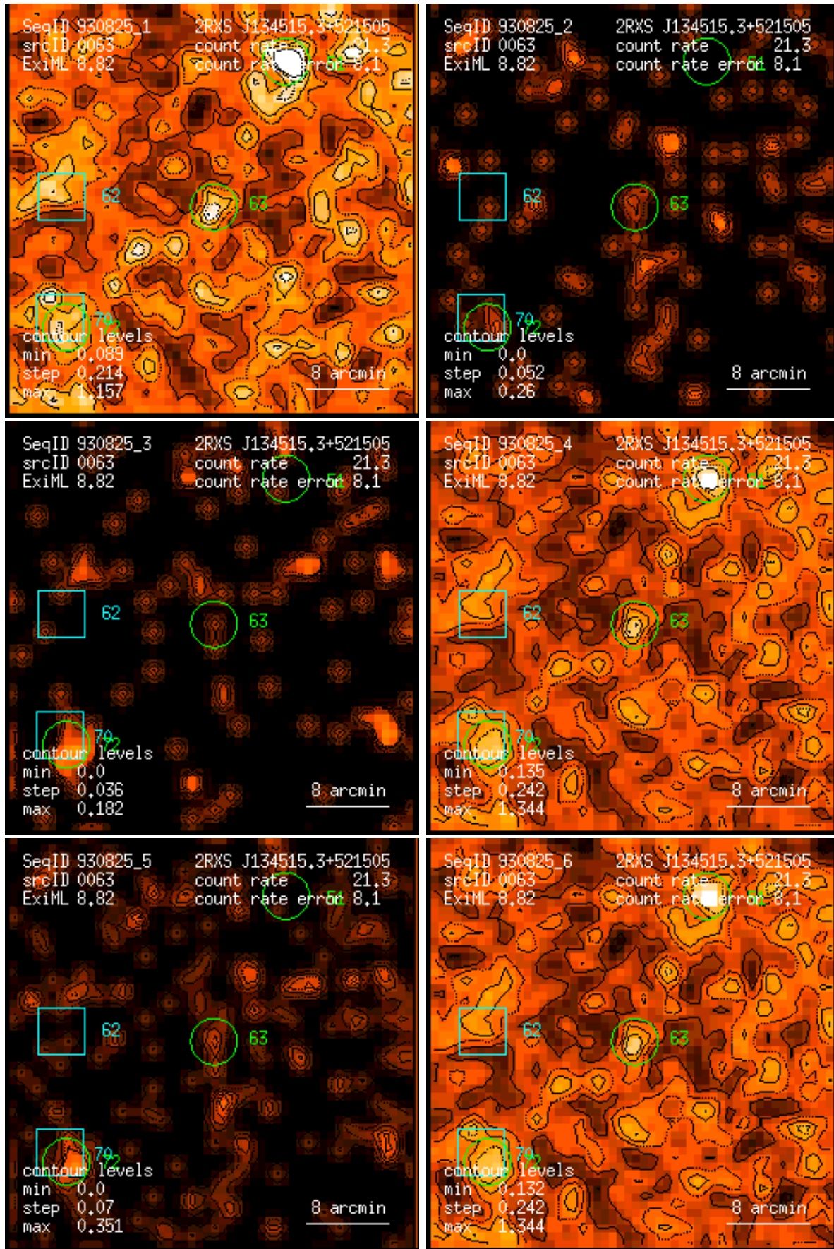
Figure 63: RASS 930825: detection 0063: band rate images, Gaussian filter: (1) PSPC channels 11 – 41, (2) 52 – 90, (3) 91 – 201, (4) 11 – 235, (5) 52 – 201, (6) 11 – 201. Broad band rates in counts/ks. Band rate contour levels in counts/ks/arcmin 2 .
