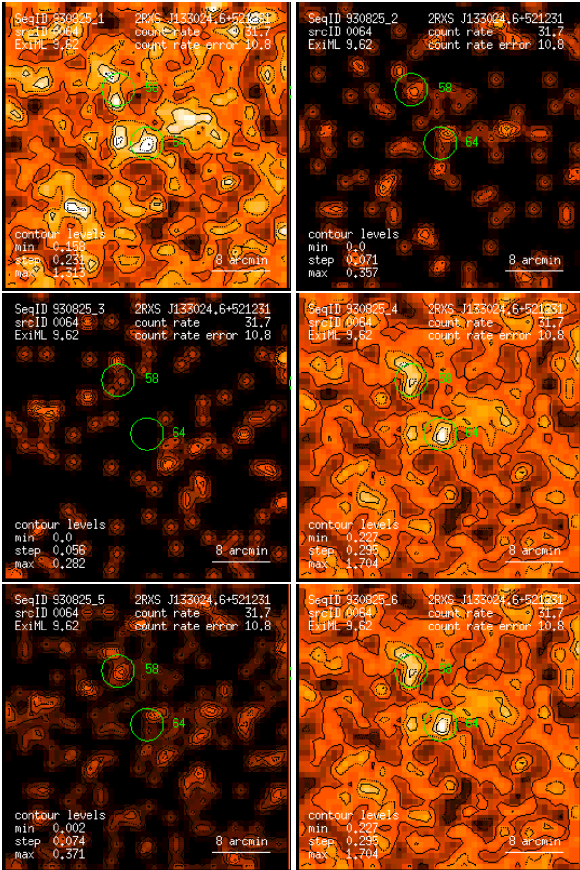
Figure 64: RASS 930825: detection 0064: band rate images, Gaussian filter: (1) PSPC channels 11 – 41, (2) 52 – 90, (3) 91 – 201, (4) 11 – 235, (5) 52 – 201, (6) 11 – 201. Broad band rates in counts/ks. Band rate contour levels in counts/ks/arcmin 2 .
