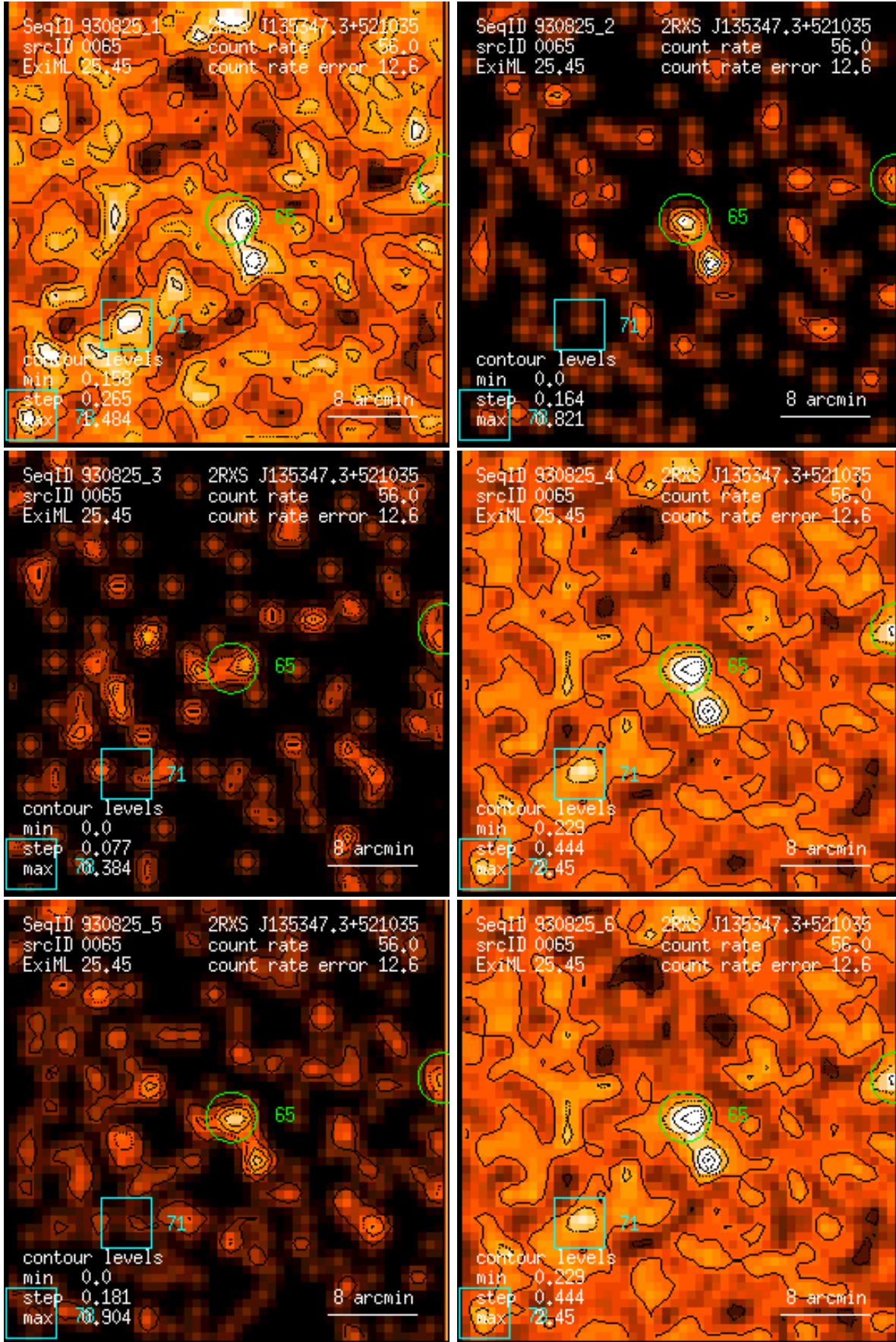
Figure 65: RASS 930825: detection 0065: band rate images, Gaussian filter: (1) PSPC channels 11 – 41, (2) 52 – 90, (3) 91 – 201, (4) 11 – 235, (5) 52 – 201, (6) 11 – 201. Broad band rates in counts/ks. Band rate contour levels in counts/ks/arcmin 2 .
