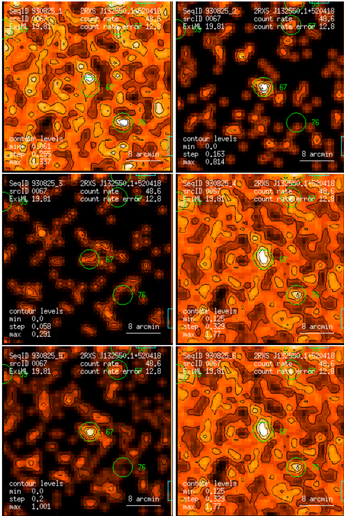
Figure 67: RASS 930825: detection 0067: band rate images, Gaussian filter: (1) PSPC channels 11 – 41, (2) 52 – 90, (3) 91 – 201, (4) 11 – 235, (5) 52 – 201, (6) 11 – 201. Broad band rates in counts/ks. Band rate contour levels in counts/ks/arcmin 2 .
