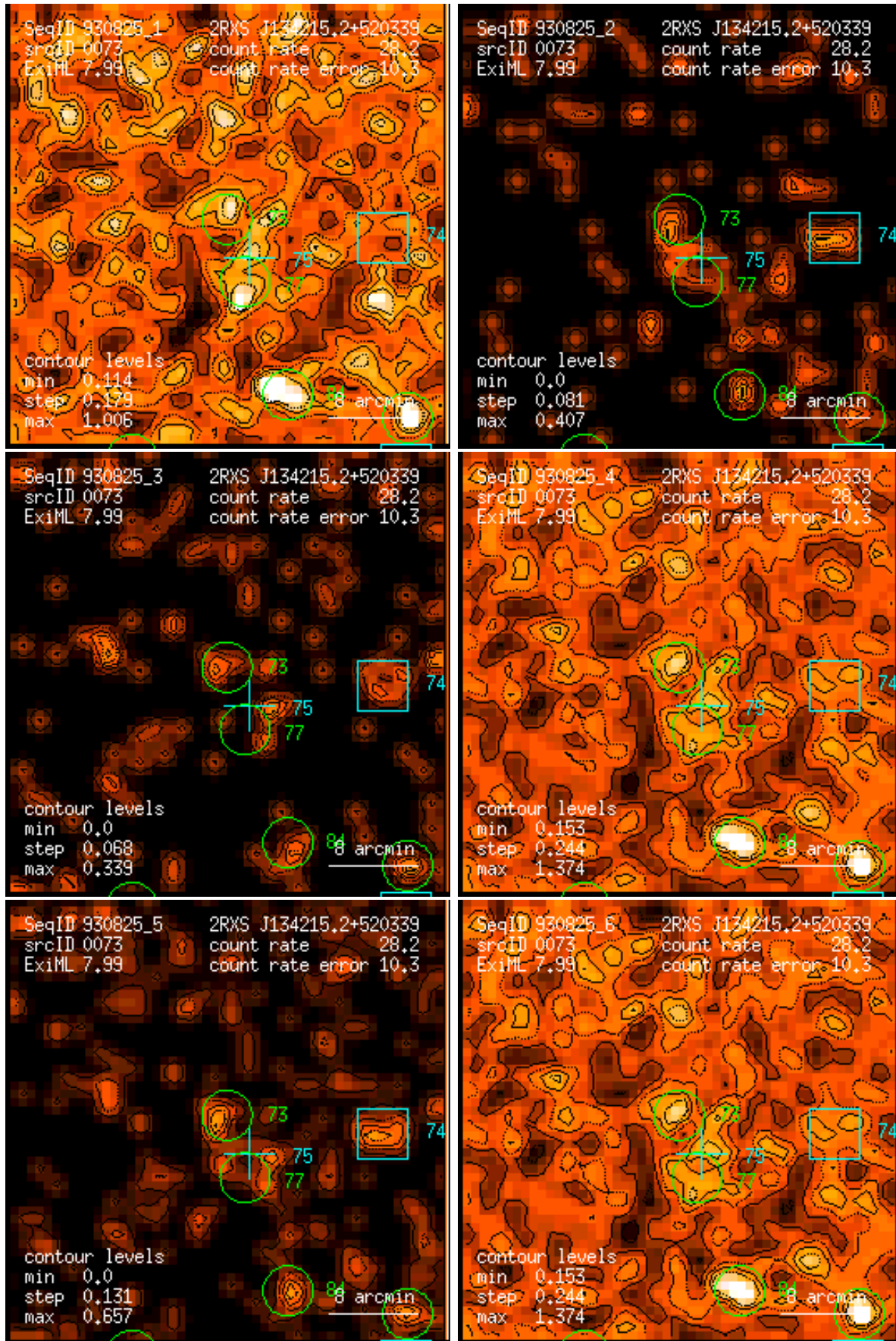
Figure 73: RASS 930825: detection 0073: band rate images, Gaussian filter: (1) PSPC channels 11 – 41, (2) 52 – 90, (3) 91 – 201, (4) 11 – 235, (5) 52 – 201, (6) 11 – 201. Broad band rates in counts/ks. Band rate contour levels in counts/ks/arcmin 2 .
