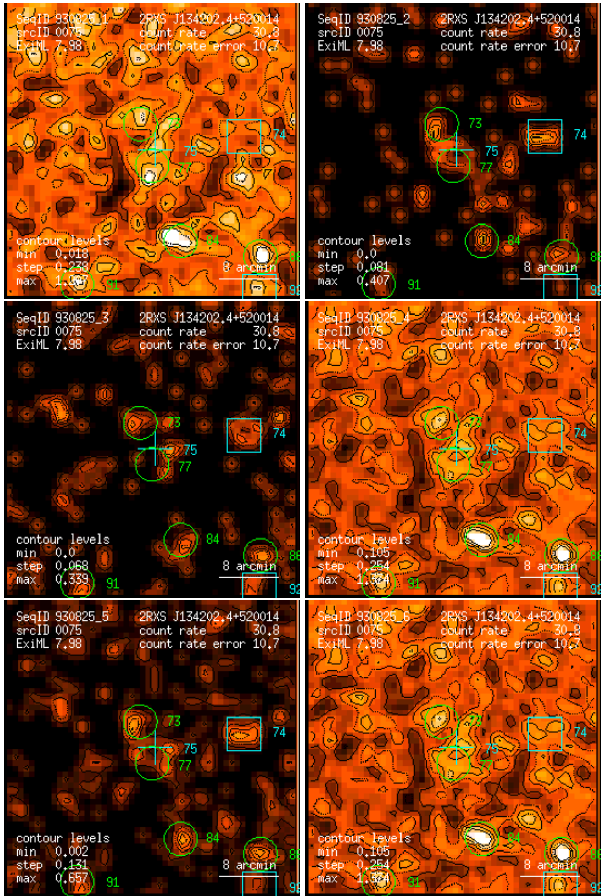
Figure 75: RASS 930825: detection 0075: band rate images, Gaussian filter: (1) PSPC channels 11 – 41, (2) 52 – 90, (3) 91 – 201, (4) 11 – 235, (5) 52 – 201, (6) 11 – 201. Broad band rates in counts/ks. Band rate contour levels in counts/ks/arcmin 2 .
