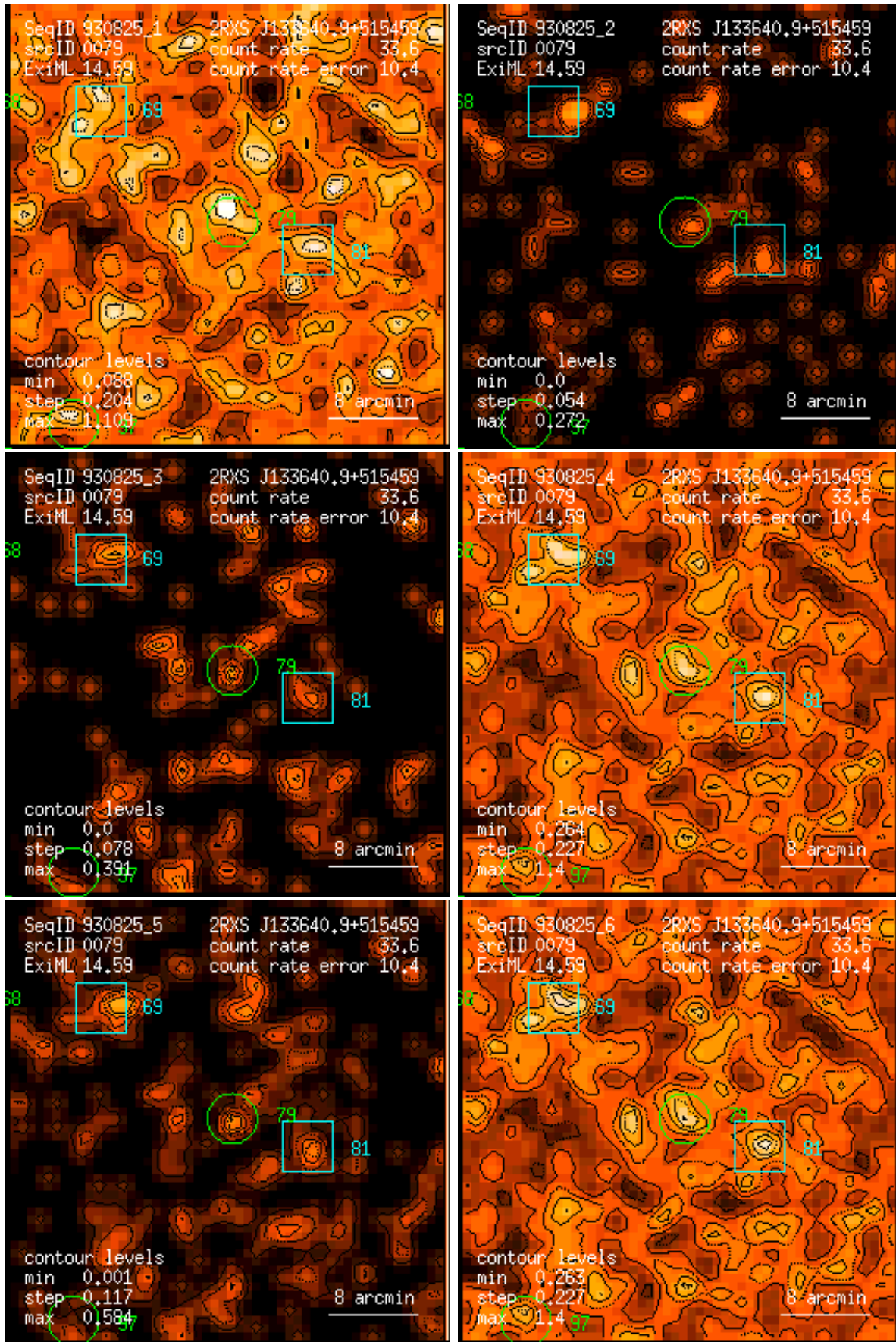
Figure 79: RASS 930825: detection 0079: band rate images, Gaussian filter: (1) PSPC channels 11 – 41, (2) 52 – 90, (3) 91 – 201, (4) 11 – 235, (5) 52 – 201, (6) 11 – 201. Broad band rates in counts/ks. Band rate contour levels in counts/ks/arcmin 2 .
