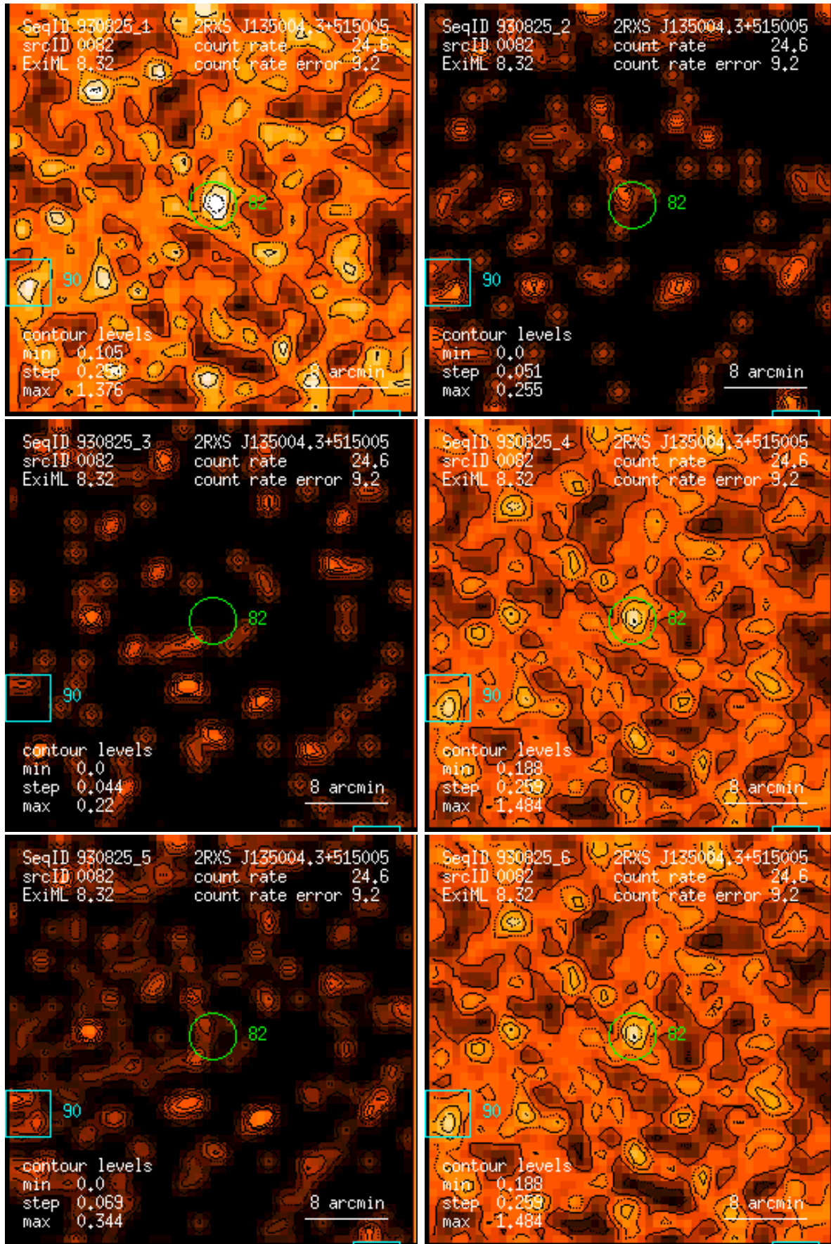
Figure 82: RASS 930825: detection 0082: band rate images, Gaussian filter: (1) PSPC channels 11 – 41, (2) 52 – 90, (3) 91 – 201, (4) 11 – 235, (5) 52 – 201, (6) 11 – 201. Broad band rates in counts/ks. Band rate contour levels in counts/ks/arcmin 2 .
