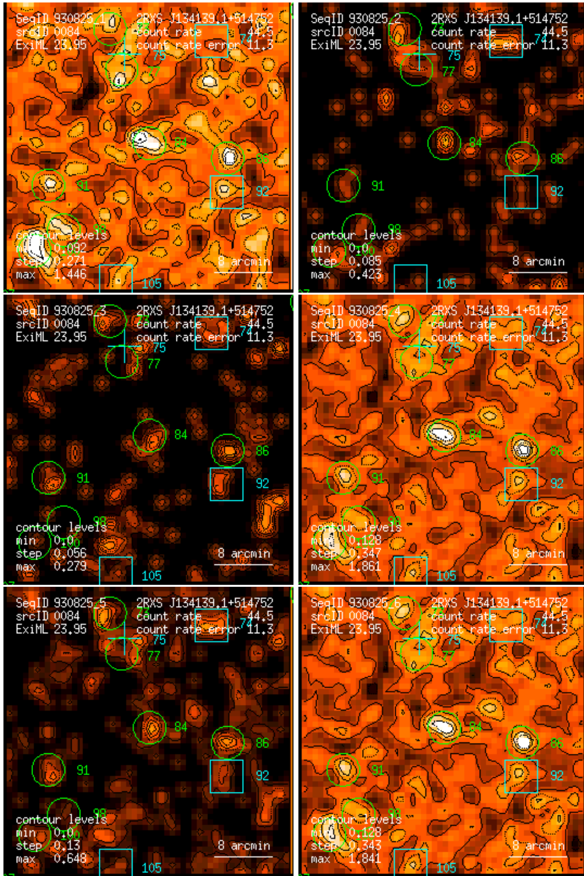
Figure 84: RASS 930825: detection 0084: band rate images, Gaussian filter: (1) PSPC channels 11 – 41, (2) 52 – 90, (3) 91 – 201, (4) 11 – 235, (5) 52 – 201, (6) 11 – 201. Broad band rates in counts/ks. Band rate contour levels in counts/ks/arcmin 2 .
