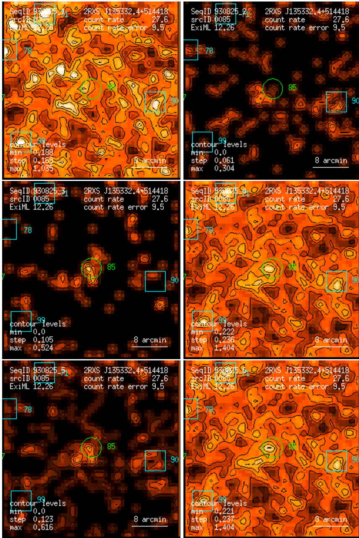
Figure 85: RASS 930825: detection 0085: band rate images, Gaussian filter: (1) PSPC channels 11 – 41, (2) 52 – 90, (3) 91 – 201, (4) 11 – 235, (5) 52 – 201, (6) 11 – 201. Broad band rates in counts/ks. Band rate contour levels in counts/ks/arcmin 2 .
