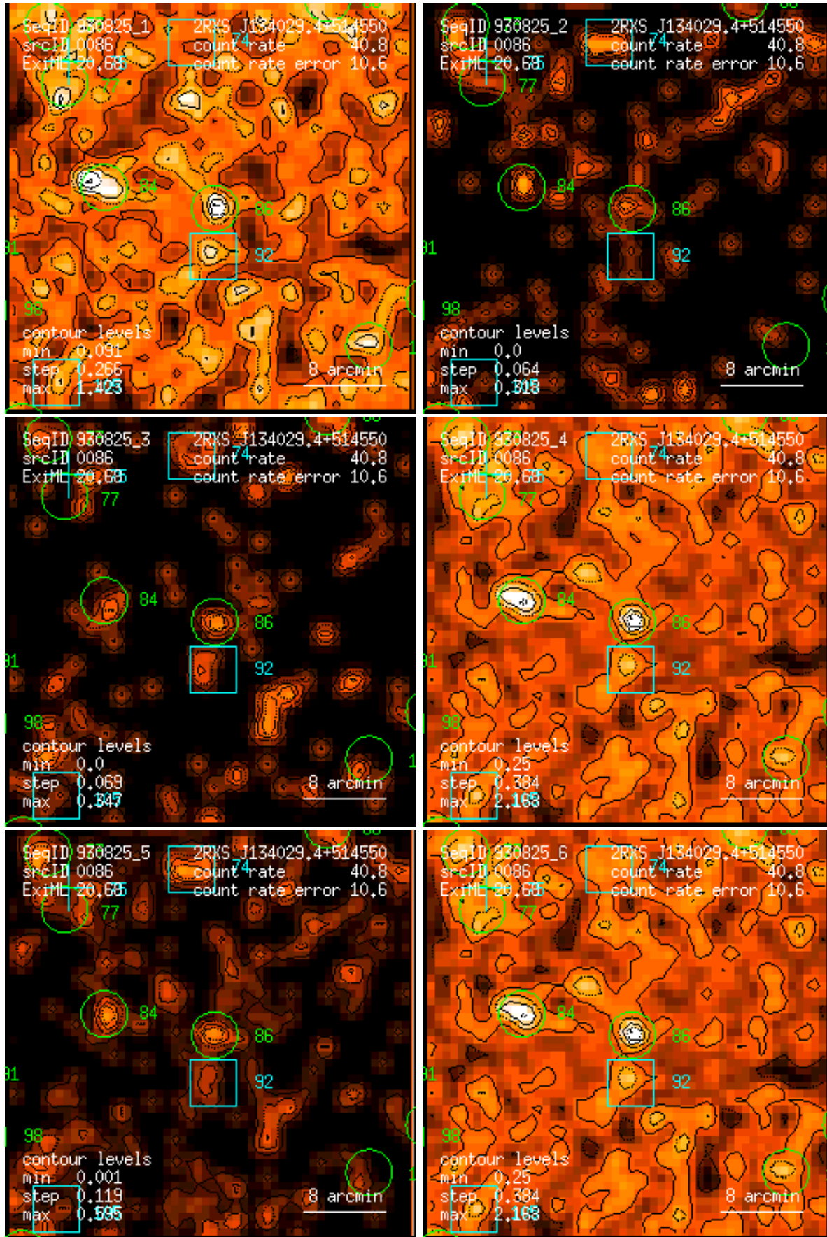
Figure 86: RASS 930825: detection 0086: band rate images, Gaussian filter: (1) PSPC channels 11 – 41, (2) 52 – 90, (3) 91 – 201, (4) 11 – 235, (5) 52 – 201, (6) 11 – 201. Broad band rates in counts/ks. Band rate contour levels in counts/ks/arcmin 2 .
