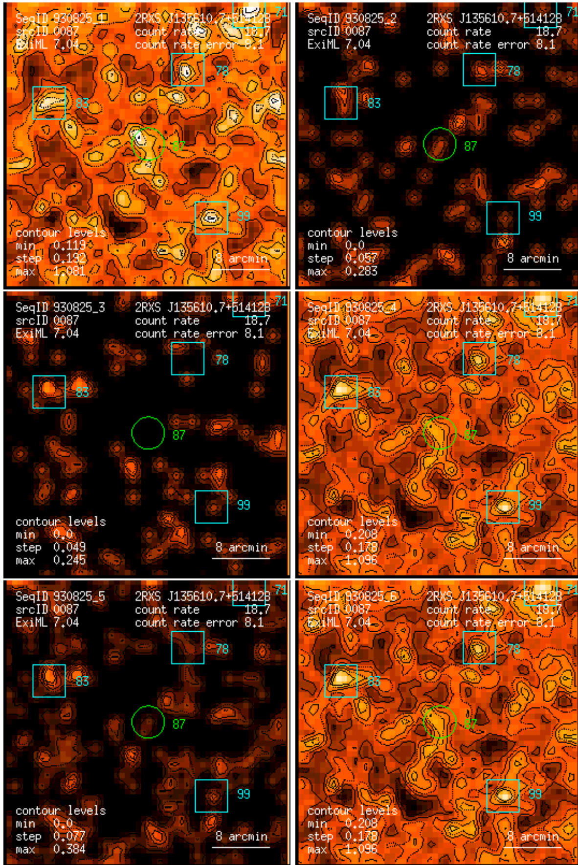
Figure 87: RASS 930825: detection 0087: band rate images, Gaussian filter: (1) PSPC channels 11 – 41, (2) 52 – 90, (3) 91 – 201, (4) 11 – 235, (5) 52 – 201, (6) 11 – 201. Broad band rates in counts/ks. Band rate contour levels in counts/ks/arcmin 2 .
