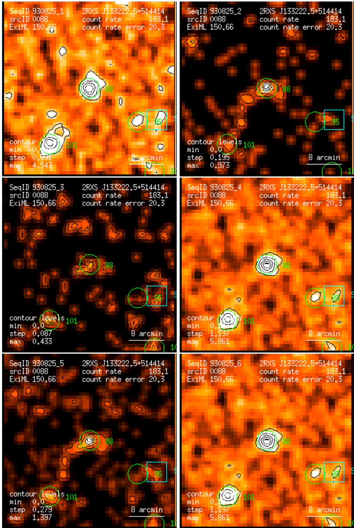
Figure 88: RASS 930825: detection 0088: band rate images, Gaussian filter: (1) PSPC channels 11 – 41, (2) 52 – 90, (3) 91 – 201, (4) 11 – 235, (5) 52 – 201, (6) 11 – 201. Broad band rates in counts/ks. Band rate contour levels in counts/ks/arcmin 2 .
