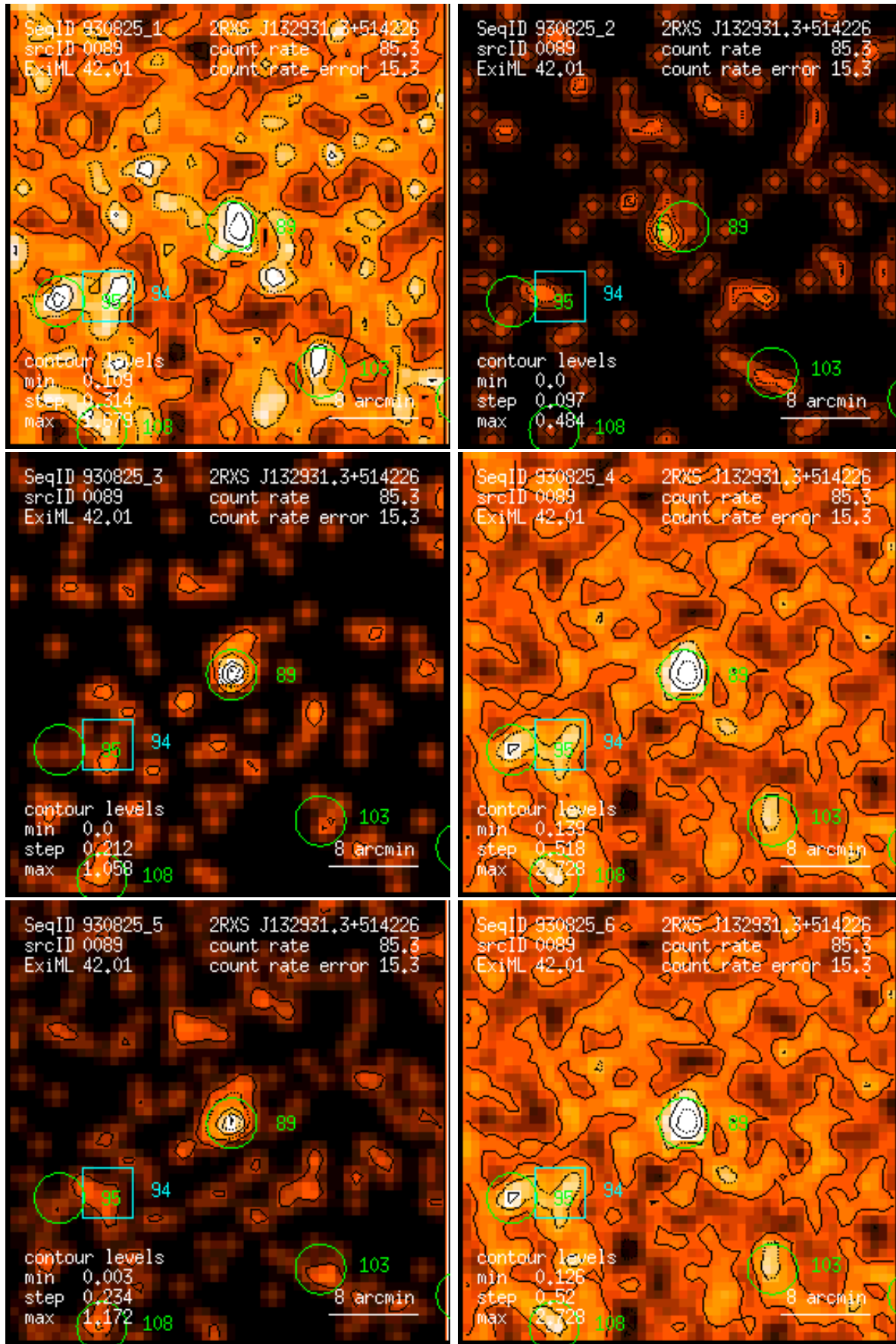
Figure 89: RASS 930825: detection 0089: band rate images, Gaussian filter: (1) PSPC channels 11 – 41, (2) 52 – 90, (3) 91 – 201, (4) 11 – 235, (5) 52 – 201, (6) 11 – 201. Broad band rates in counts/ks. Band rate contour levels in counts/ks/arcmin 2 .
