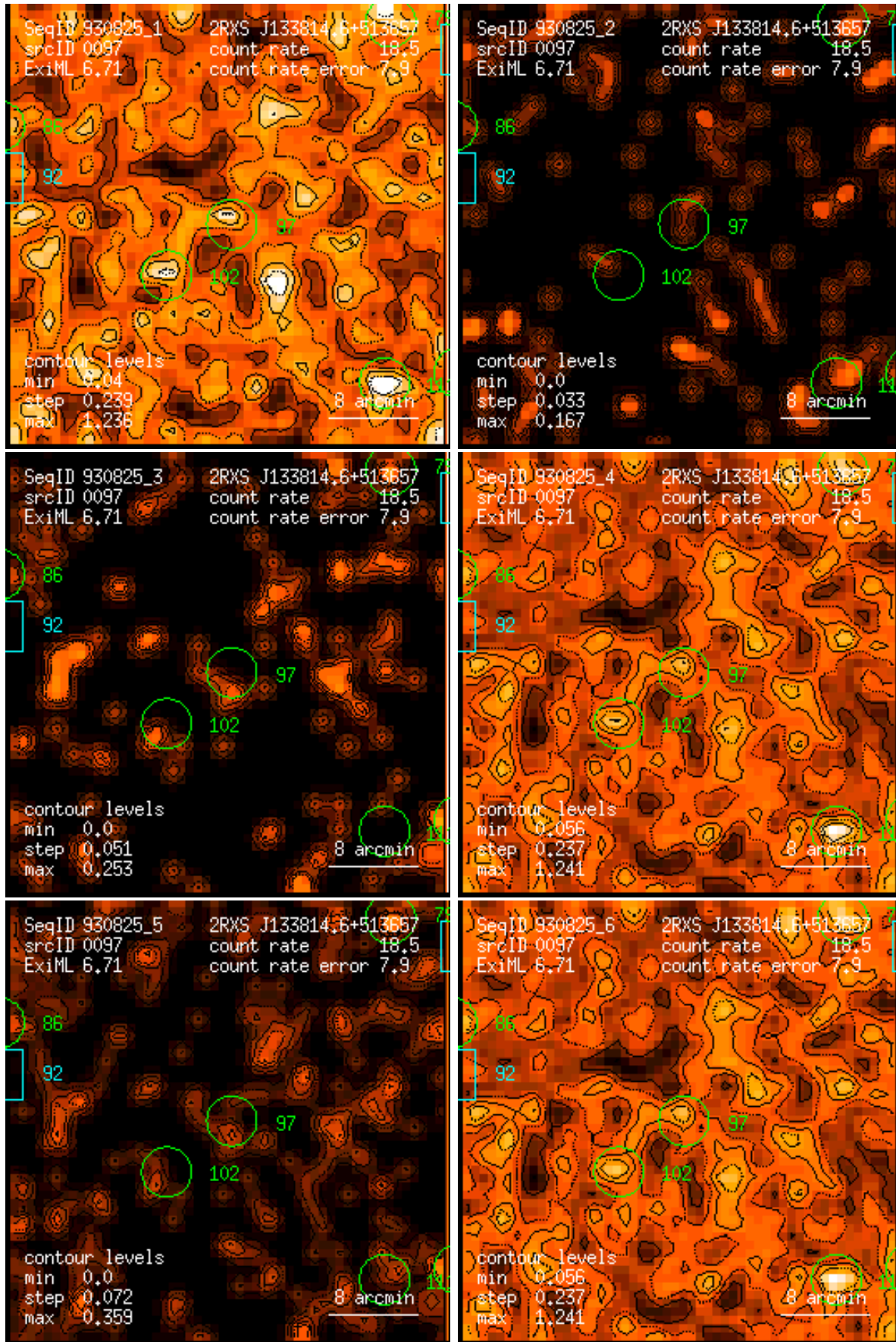
Figure 97: RASS 930825: detection 0097: band rate images, Gaussian filter: (1) PSPC channels 11 – 41, (2) 52 – 90, (3) 91 – 201, (4) 11 – 235, (5) 52 – 201, (6) 11 – 201. Broad band rates in counts/ks. Band rate contour levels in counts/ks/arcmin 2 .
