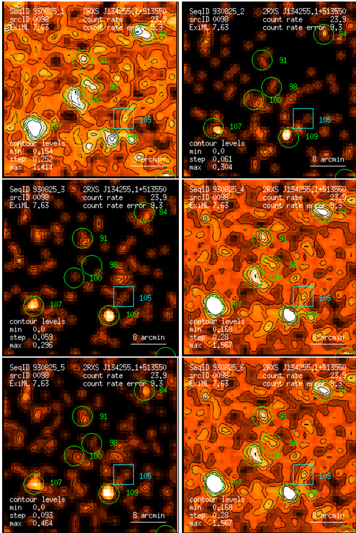
Figure 98: RASS 930825: detection 0098: band rate images, Gaussian filter: (1) PSPC channels 11 – 41, (2) 52 – 90, (3) 91 – 201, (4) 11 – 235, (5) 52 – 201, (6) 11 – 201. Broad band rates in counts/ks. Band rate contour levels in counts/ks/arcmin 2 .
