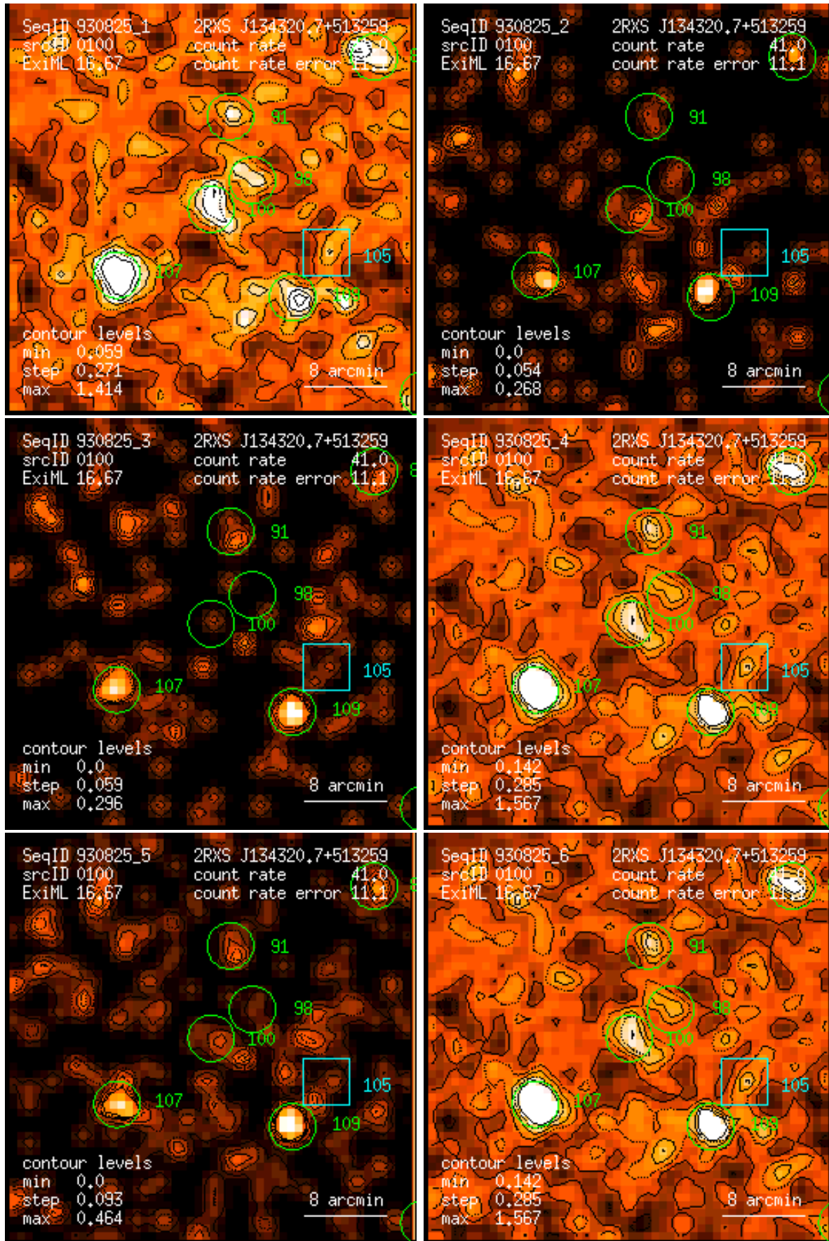
Figure 100: RASS 930825: detection 0100: band rate images, Gaussian filter: (1) PSPC channels 11 – 41, (2) 52 – 90, (3) 91 – 201, (4) 11 – 235, (5) 52 – 201, (6) 11 – 201. Broad band rates in counts/ks. Band rate contour levels in counts/ks/arcmin 2 .
