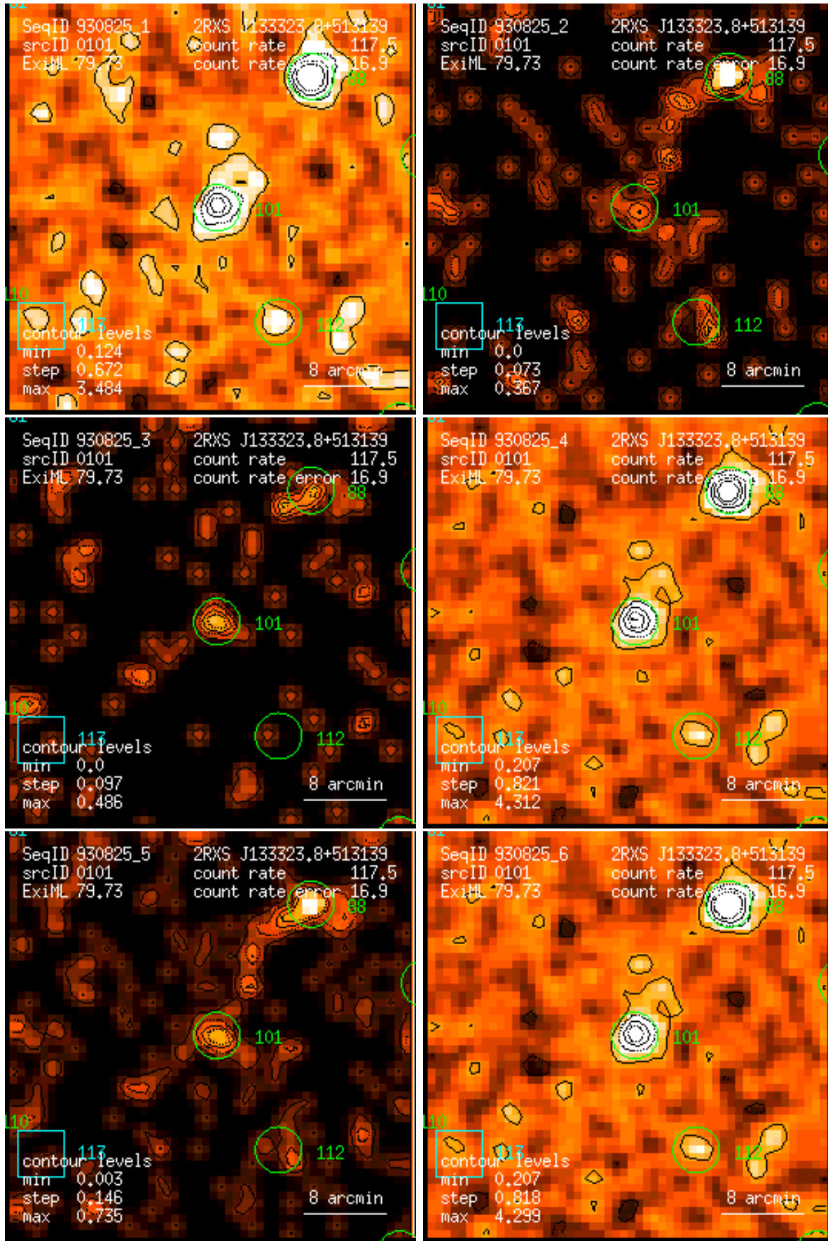
Figure 101: RASS 930825: detection 0101: band rate images, Gaussian filter: (1) PSPC channels 11 – 41, (2) 52 – 90, (3) 91 – 201, (4) 11 – 235, (5) 52 – 201, (6) 11 – 201. Broad band rates in counts/ks. Band rate contour levels in counts/ks/arcmin 2 .
