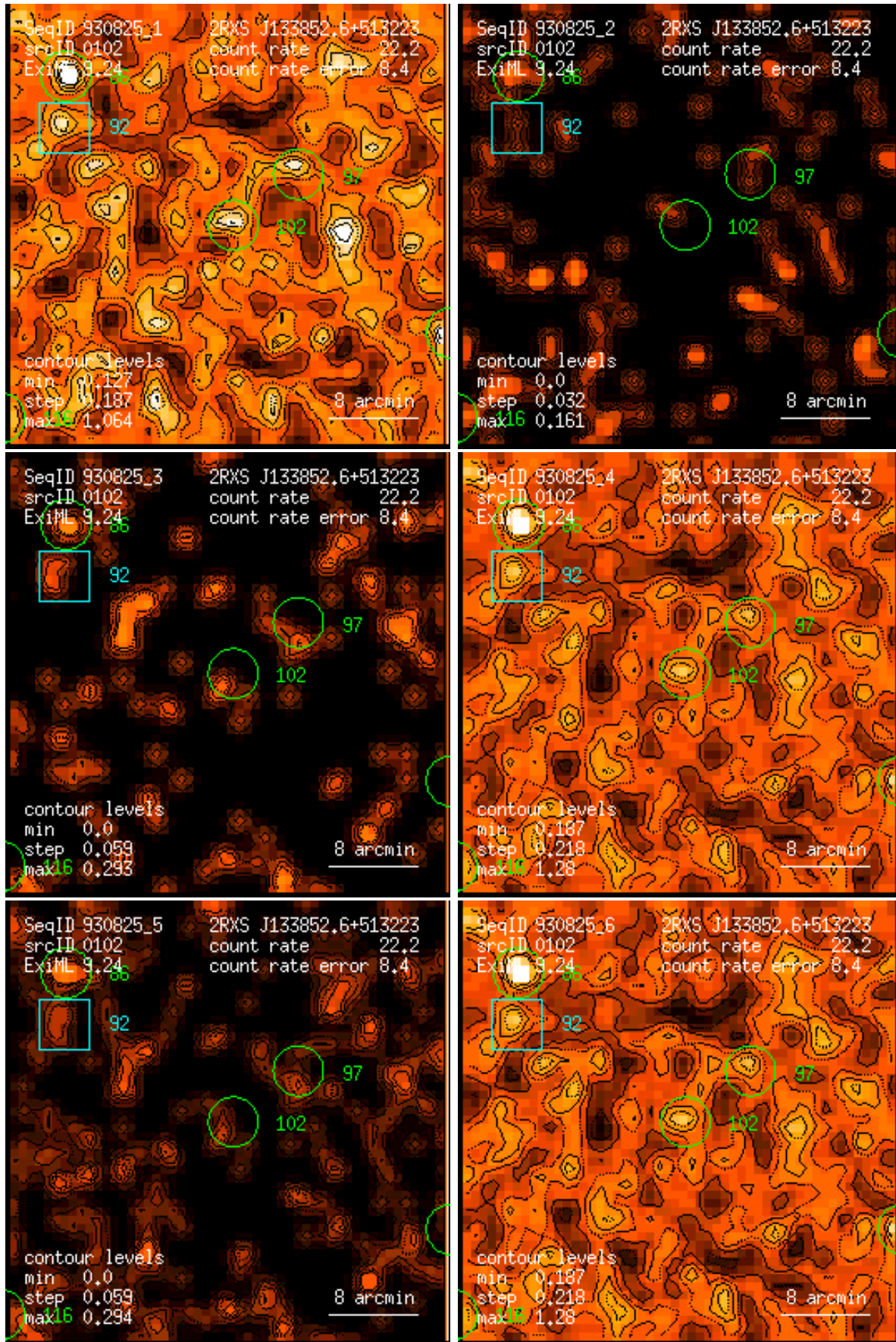
Figure 102: RASS 930825: detection 0102: band rate images, Gaussian filter: (1) PSPC channels 11 – 41, (2) 52 – 90, (3) 91 – 201, (4) 11 – 235, (5) 52 – 201, (6) 11 – 201. Broad band rates in counts/ks. Band rate contour levels in counts/ks/arcmin 2 .
