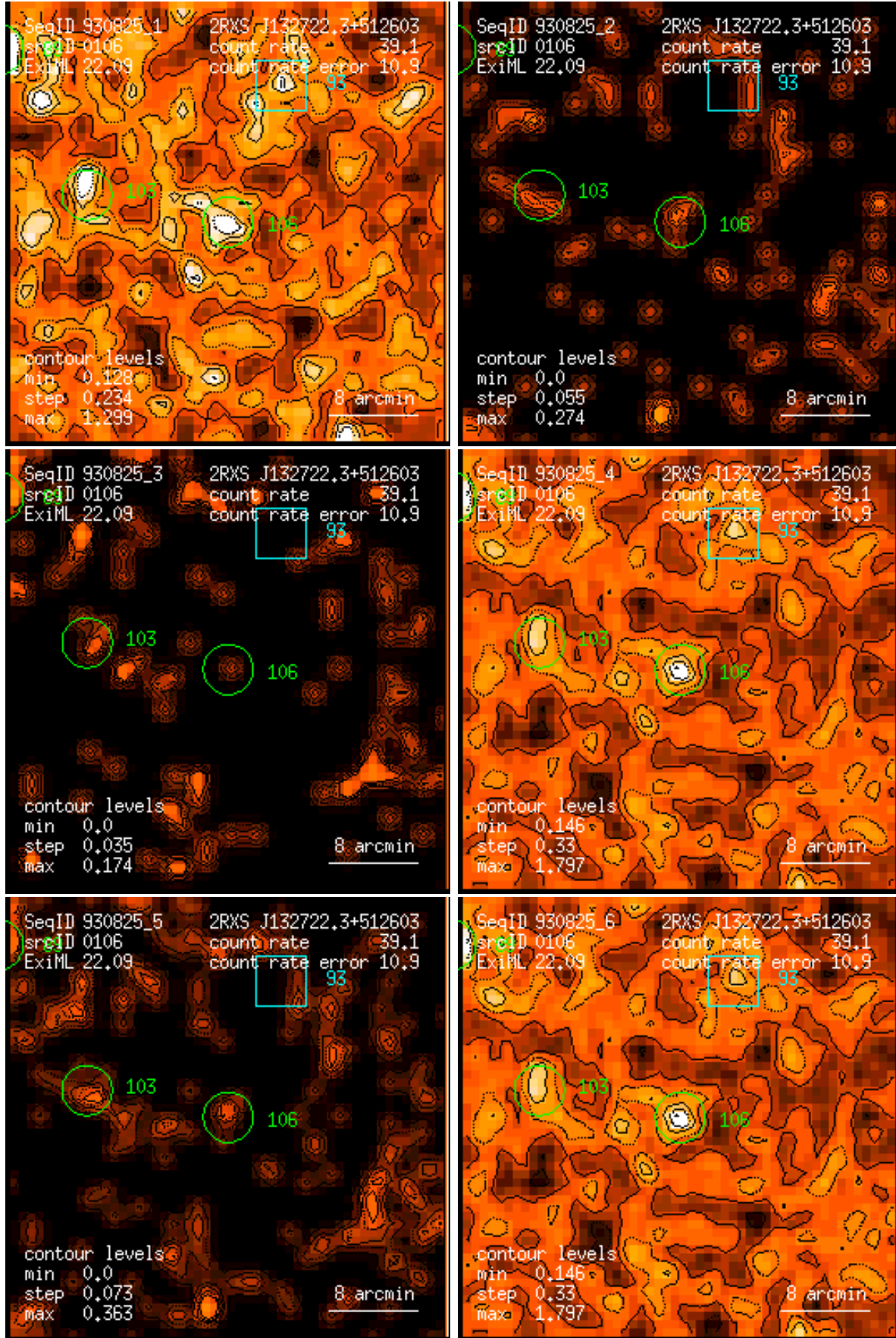
Figure 106: RASS 930825: detection 0106: band rate images, Gaussian filter: (1) PSPC channels 11 – 41, (2) 52 – 90, (3) 91 – 201, (4) 11 – 235, (5) 52 – 201, (6) 11 – 201. Broad band rates in counts/ks. Band rate contour levels in counts/ks/arcmin 2 .
