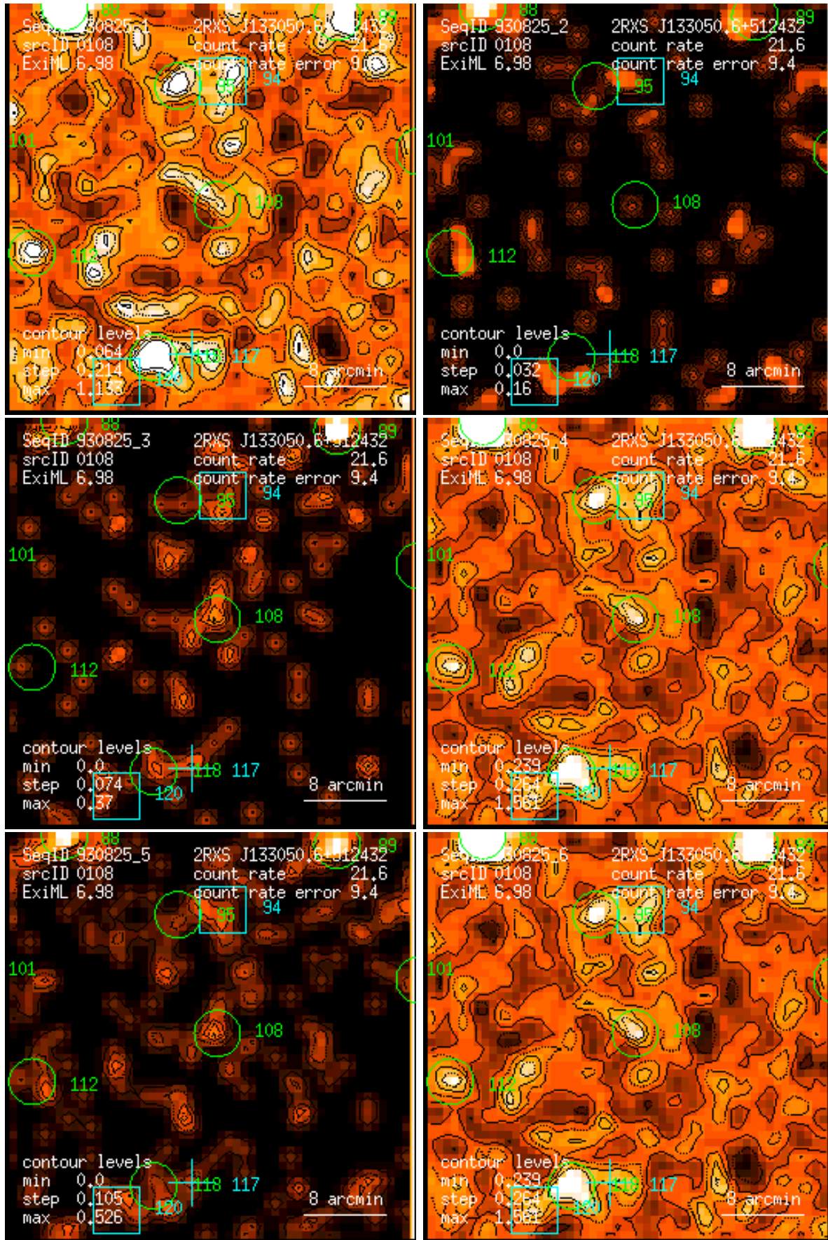
Figure 108: RASS 930825: detection 0108: band rate images, Gaussian filter: (1) PSPC channels 11 – 41, (2) 52 – 90, (3) 91 – 201, (4) 11 – 235, (5) 52 – 201, (6) 11 – 201. Broad band rates in counts/ks. Band rate contour levels in counts/ks/arcmin 2 .
