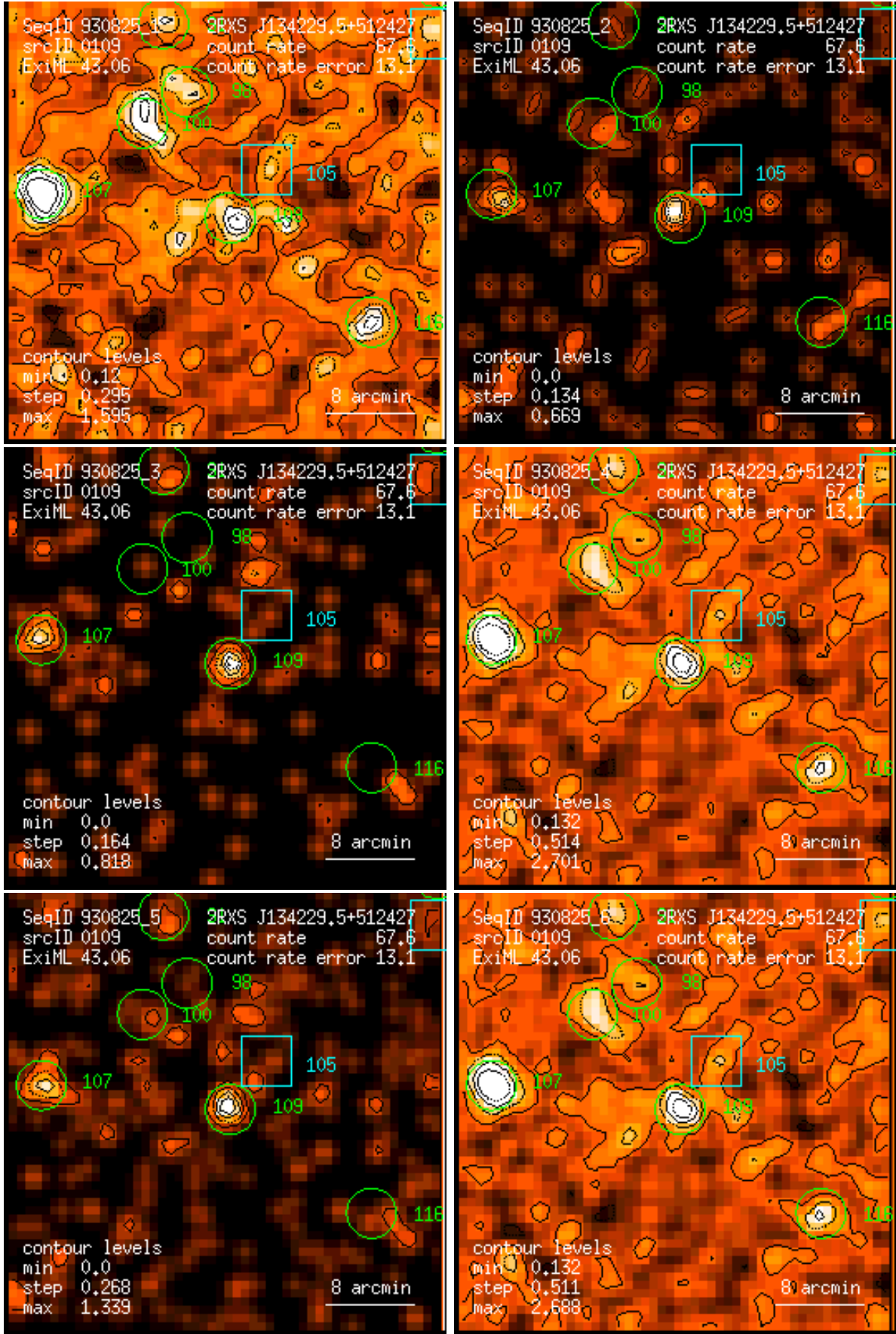
Figure 109: RASS 930825: detection 0109: band rate images, Gaussian filter: (1) PSPC channels 11 – 41, (2) 52 – 90, (3) 91 – 201, (4) 11 – 235, (5) 52 – 201, (6) 11 – 201. Broad band rates in counts/ks. Band rate contour levels in counts/ks/arcmin 2 .
