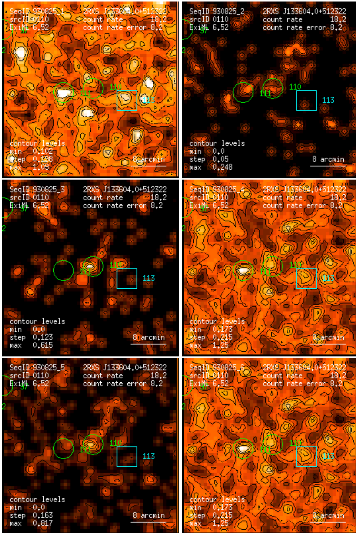
Figure 110: RASS 930825: detection 0110: band rate images, Gaussian filter: (1) PSPC channels 11 – 41, (2) 52 – 90, (3) 91 – 201, (4) 11 – 235, (5) 52 – 201, (6) 11 – 201. Broad band rates in counts/ks. Band rate contour levels in counts/ks/arcmin 2 .
