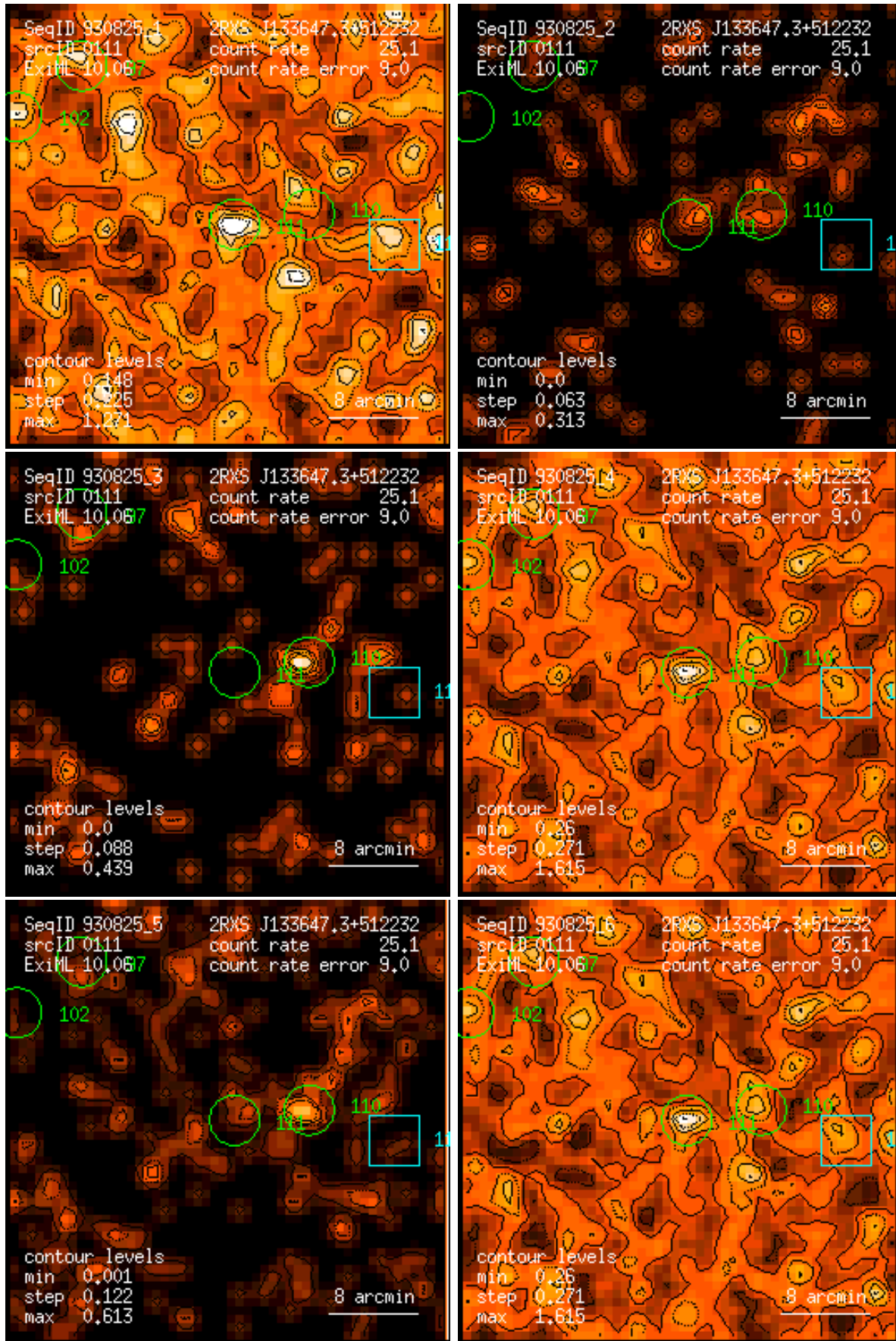
Figure 111: RASS 930825: detection 0111: band rate images, Gaussian filter: (1) PSPC channels 11 – 41, (2) 52 – 90, (3) 91 – 201, (4) 11 – 235, (5) 52 – 201, (6) 11 – 201. Broad band rates in counts/ks. Band rate contour levels in counts/ks/arcmin 2 .
