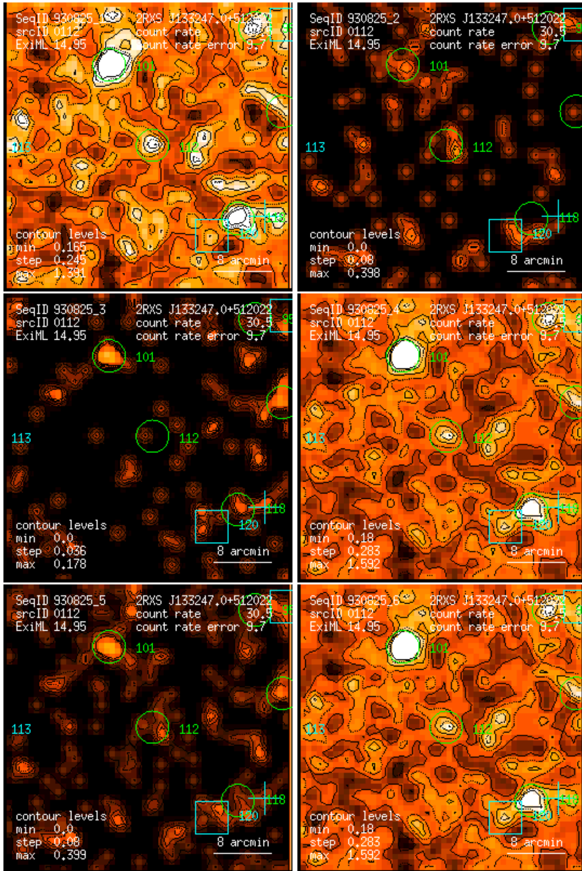
Figure 112: RASS 930825: detection 0112: band rate images, Gaussian filter: (1) PSPC channels 11 – 41, (2) 52 – 90, (3) 91 – 201, (4) 11 – 235, (5) 52 – 201, (6) 11 – 201. Broad band rates in counts/ks. Band rate contour levels in counts/ks/arcmin 2 .
