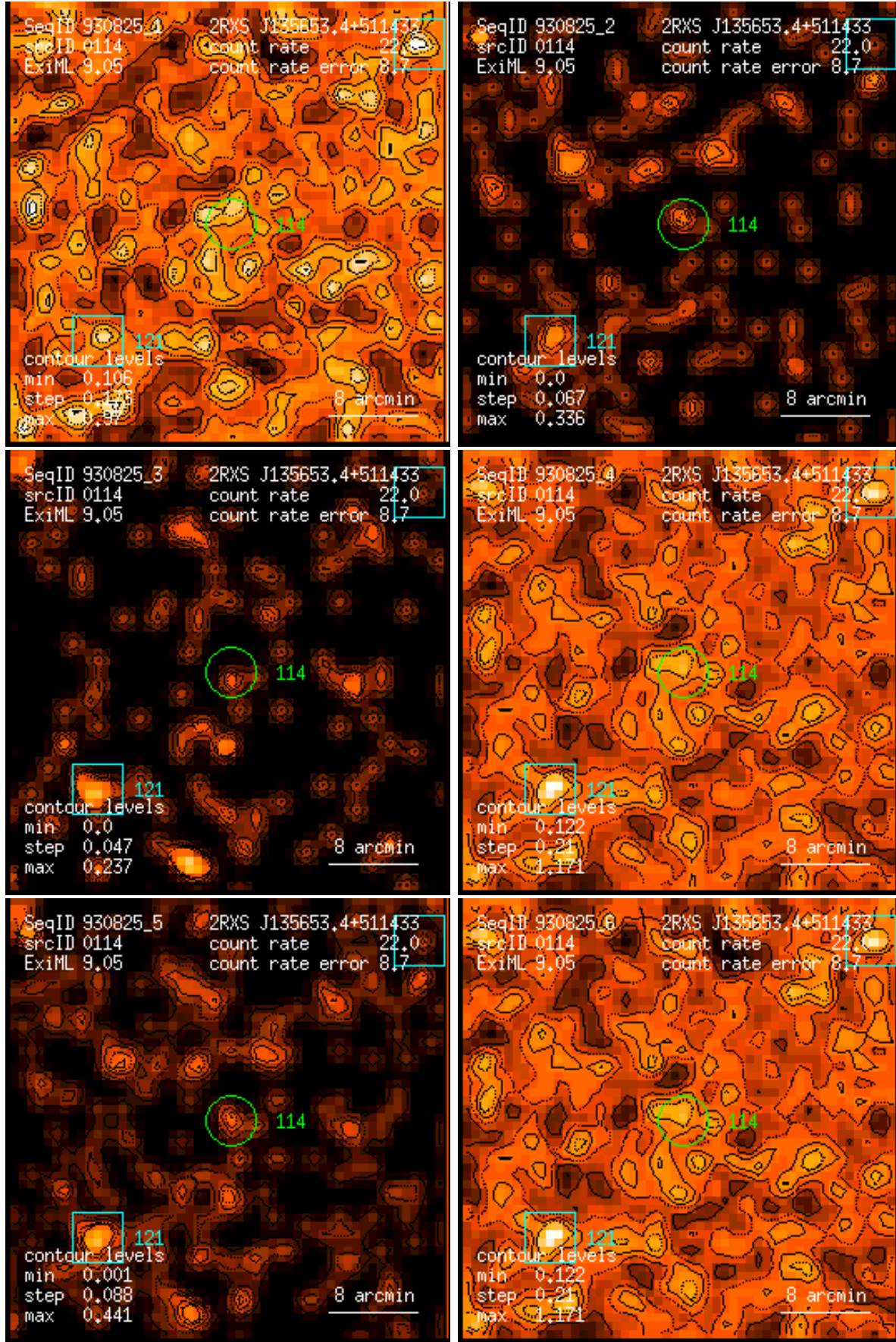
Figure 114: RASS 930825: detection 0114: band rate images, Gaussian filter: (1) PSPC channels 11 – 41, (2) 52 – 90, (3) 91 – 201, (4) 11 – 235, (5) 52 – 201, (6) 11 – 201. Broad band rates in counts/ks. Band rate contour levels in counts/ks/arcmin 2 .
