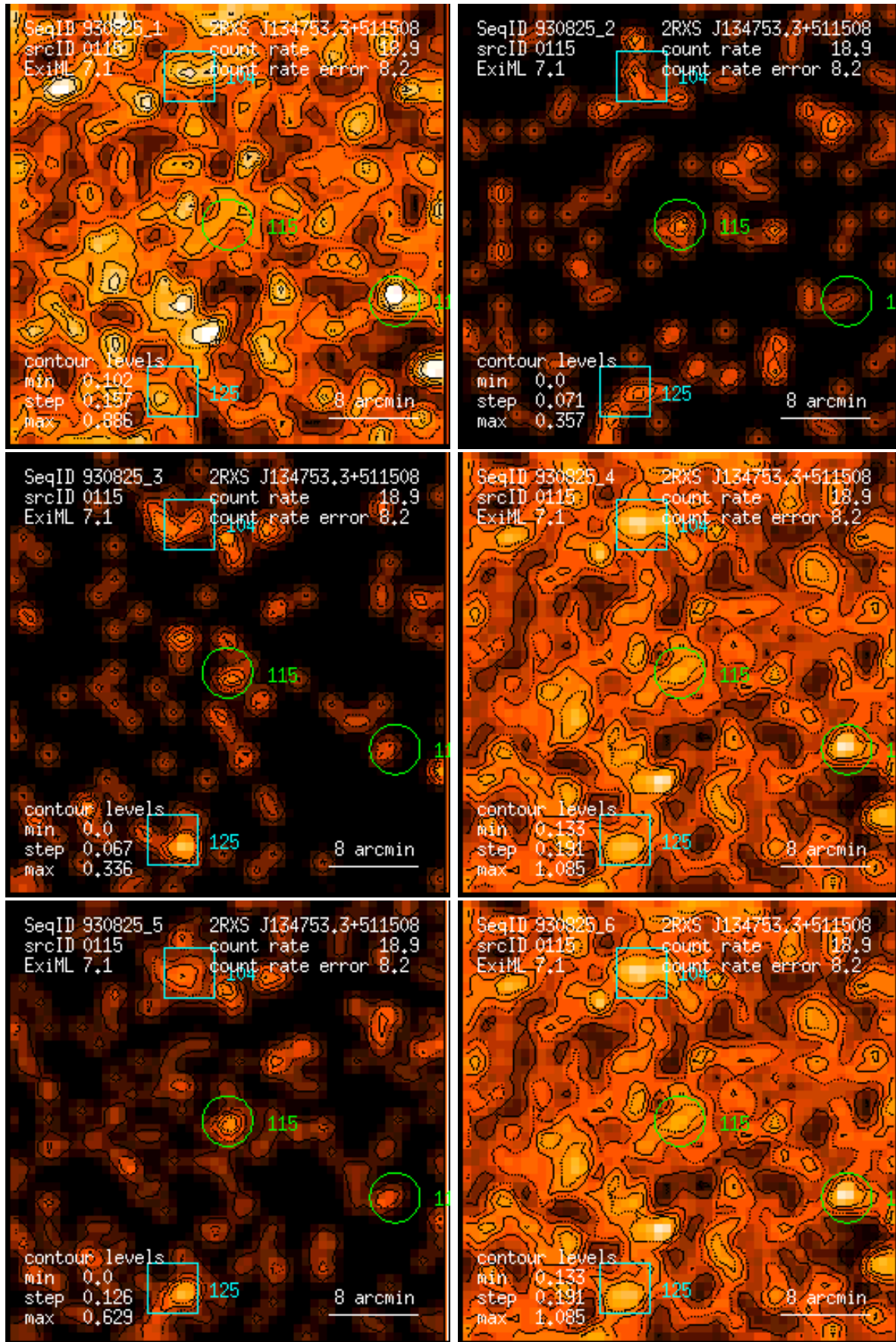
Figure 115: RASS 930825: detection 0115: band rate images, Gaussian filter: (1) PSPC channels 11 – 41, (2) 52 – 90, (3) 91 – 201, (4) 11 – 235, (5) 52 – 201, (6) 11 – 201. Broad band rates in counts/ks. Band rate contour levels in counts/ks/arcmin 2 .
