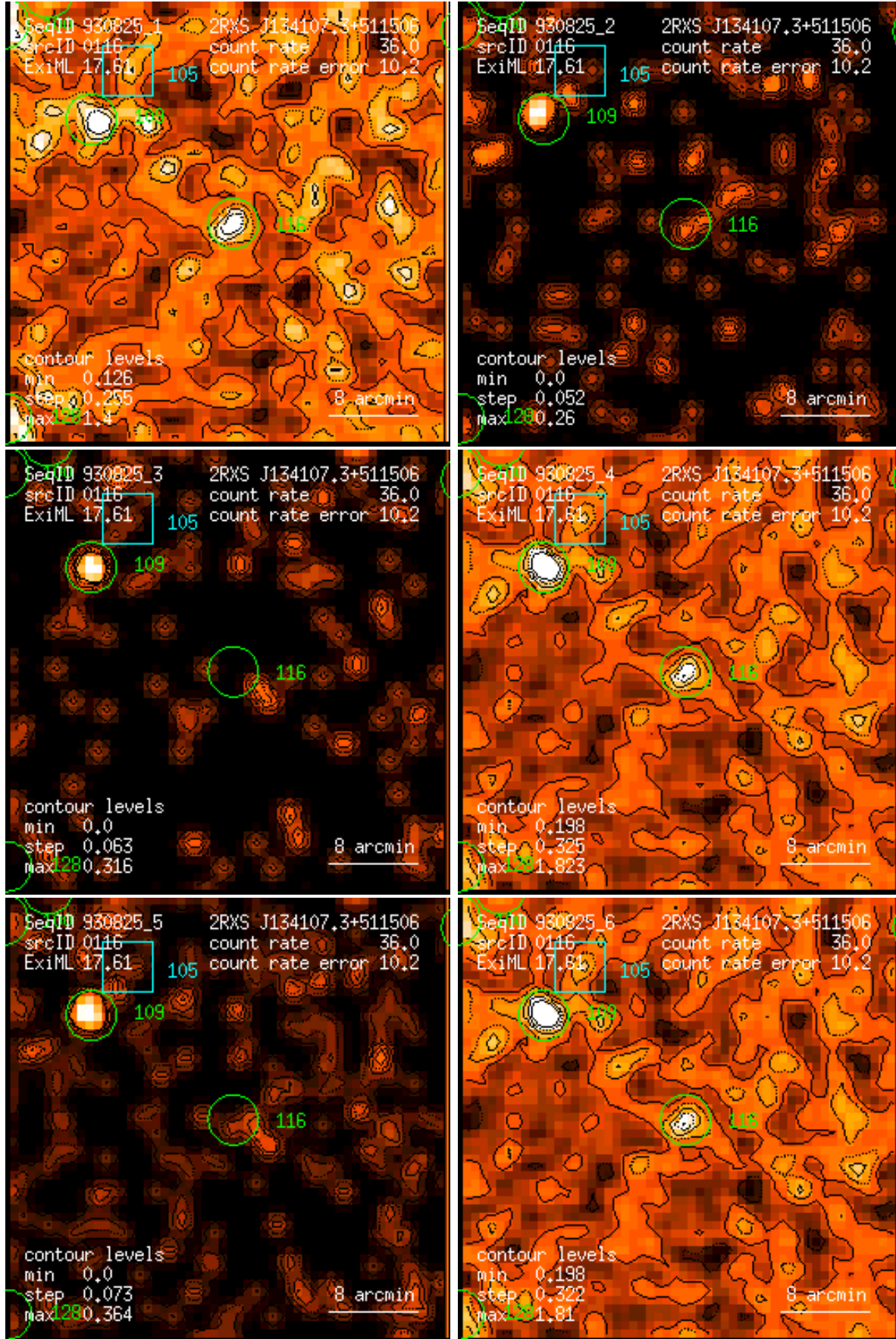
Figure 116: RASS 930825: detection 0116: band rate images, Gaussian filter: (1) PSPC channels 11 – 41, (2) 52 – 90, (3) 91 – 201, (4) 11 – 235, (5) 52 – 201, (6) 11 – 201. Broad band rates in counts/ks. Band rate contour levels in counts/ks/arcmin 2 .
