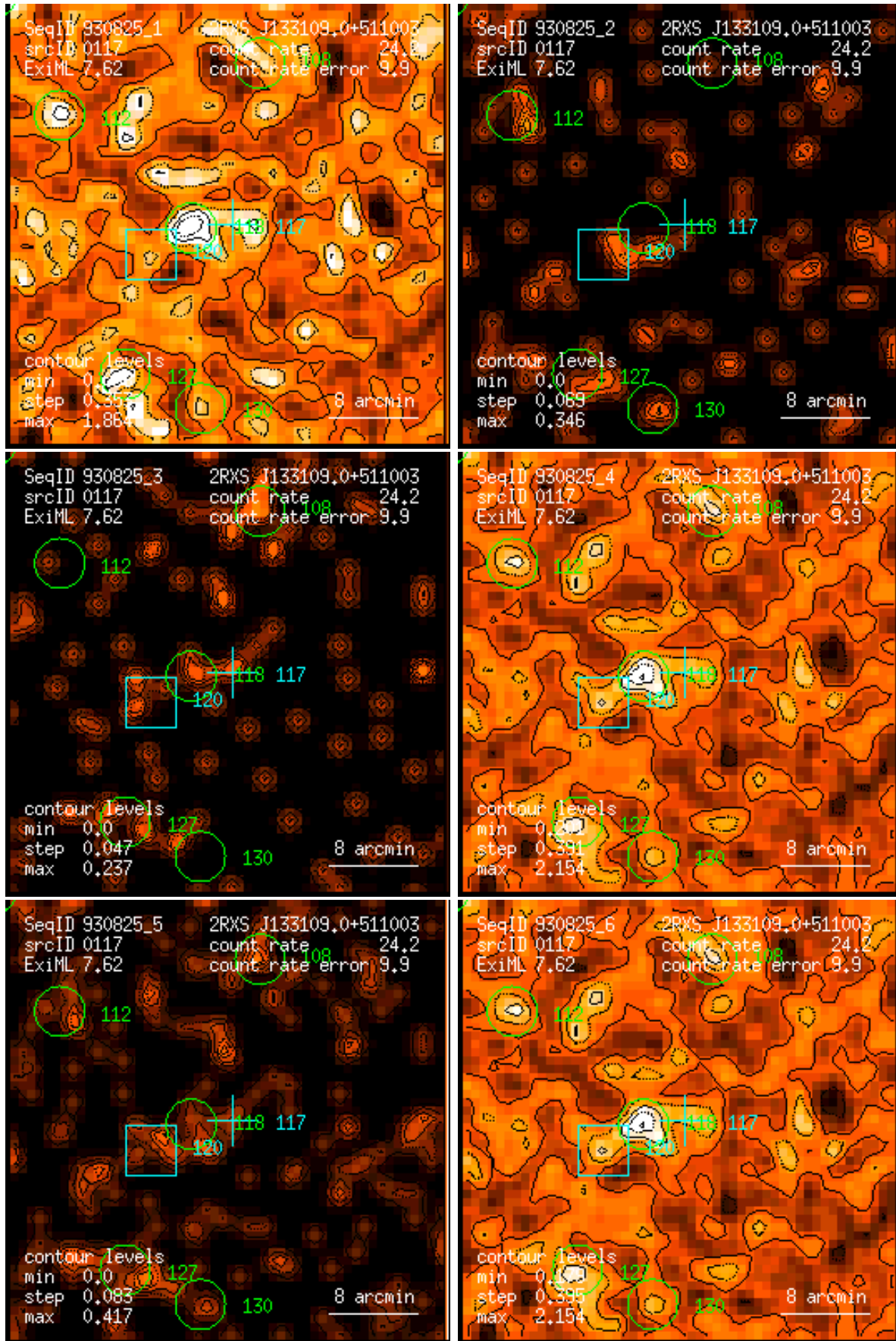
Figure 117: RASS 930825: detection 0117: band rate images, Gaussian filter: (1) PSPC channels 11 – 41, (2) 52 – 90, (3) 91 – 201, (4) 11 – 235, (5) 52 – 201, (6) 11 – 201. Broad band rates in counts/ks. Band rate contour levels in counts/ks/arcmin 2 .
