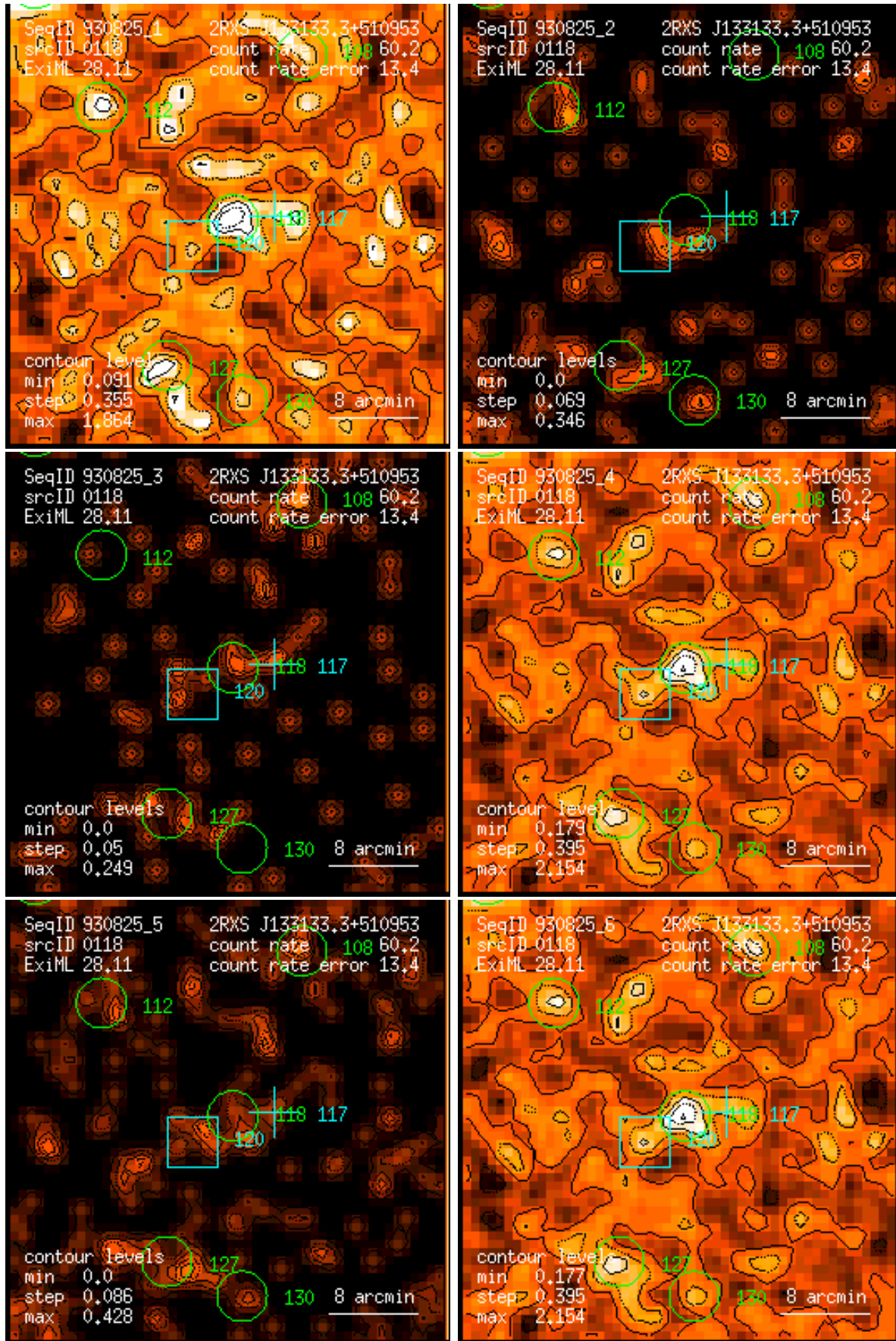
Figure 118: RASS 930825: detection 0118: band rate images, Gaussian filter: (1) PSPC channels 11 – 41, (2) 52 – 90, (3) 91 – 201, (4) 11 – 235, (5) 52 – 201, (6) 11 – 201. Broad band rates in counts/ks. Band rate contour levels in counts/ks/arcmin 2 .
