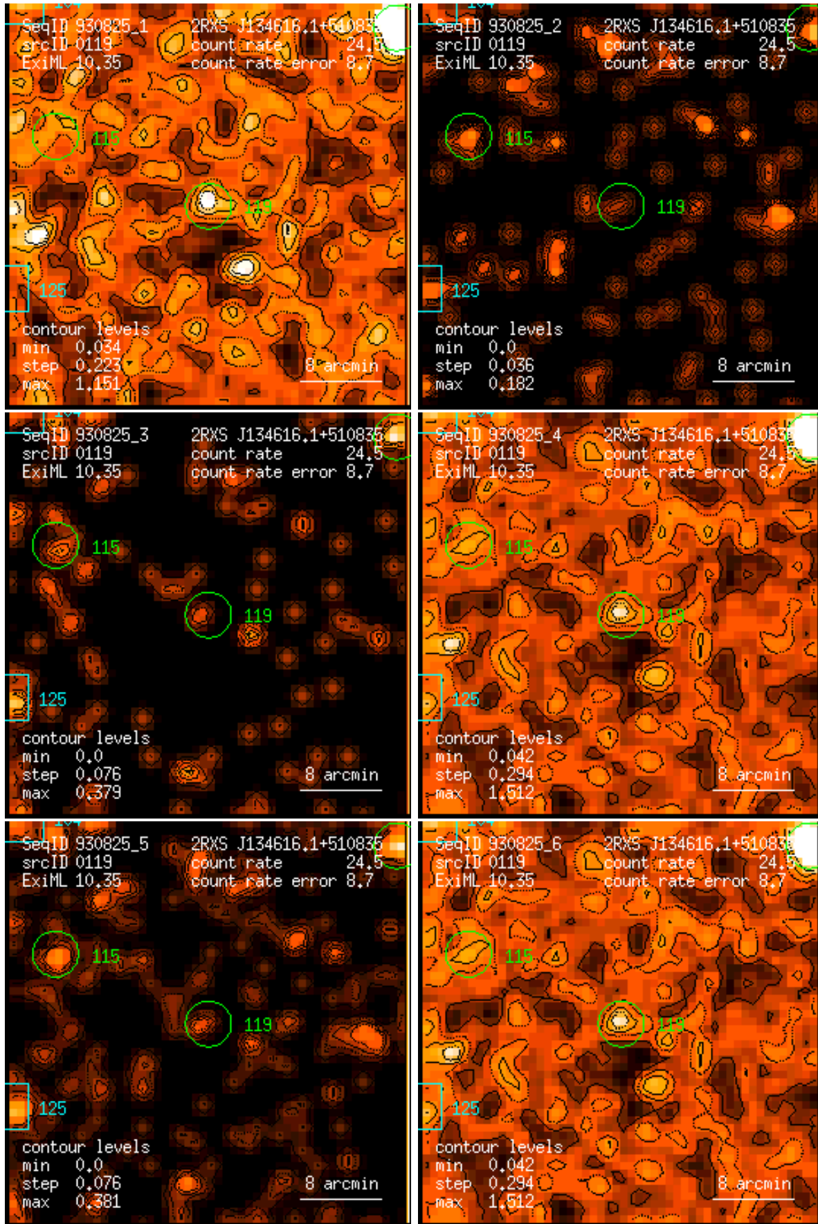
Figure 119: RASS 930825: detection 0119: band rate images, Gaussian filter: (1) PSPC channels 11 – 41, (2) 52 – 90, (3) 91 – 201, (4) 11 – 235, (5) 52 – 201, (6) 11 – 201. Broad band rates in counts/ks. Band rate contour levels in counts/ks/arcmin 2 .
