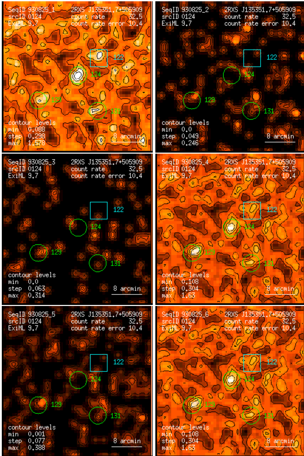
Figure 124: RASS 930825: detection 0124: band rate images, Gaussian filter: (1) PSPC channels 11 – 41, (2) 52 – 90, (3) 91 – 201, (4) 11 – 235, (5) 52 – 201, (6) 11 – 201. Broad band rates in counts/ks. Band rate contour levels in counts/ks/arcmin 2 .
