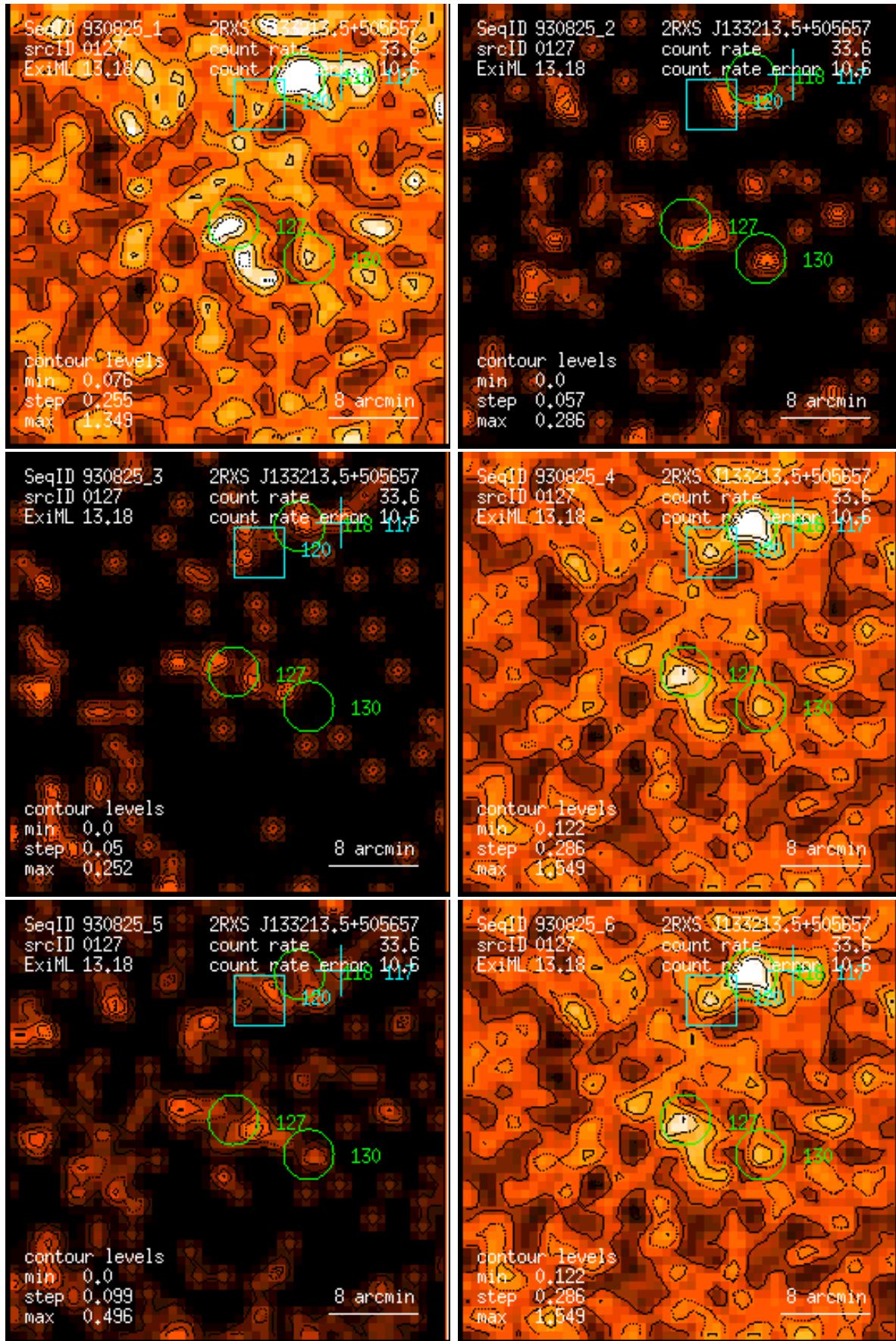
Figure 127: RASS 930825: detection 0127: band rate images, Gaussian filter: (1) PSPC channels 11 – 41, (2) 52 – 90, (3) 91 – 201, (4) 11 – 235, (5) 52 – 201, (6) 11 – 201. Broad band rates in counts/ks. Band rate contour levels in counts/ks/arcmin 2 .
