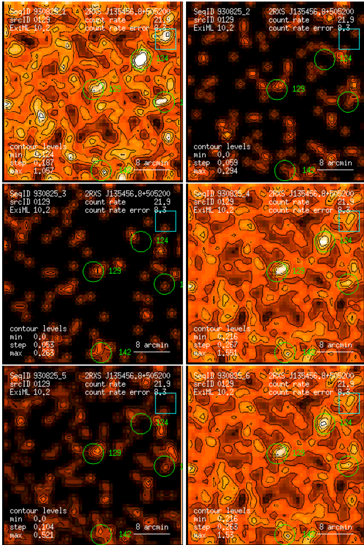
Figure 129: RASS 930825: detection 0129: band rate images, Gaussian filter: (1) PSPC channels 11 – 41, (2) 52 – 90, (3) 91 – 201, (4) 11 – 235, (5) 52 – 201, (6) 11 – 201. Broad band rates in counts/ks. Band rate contour levels in counts/ks/arcmin 2 .
