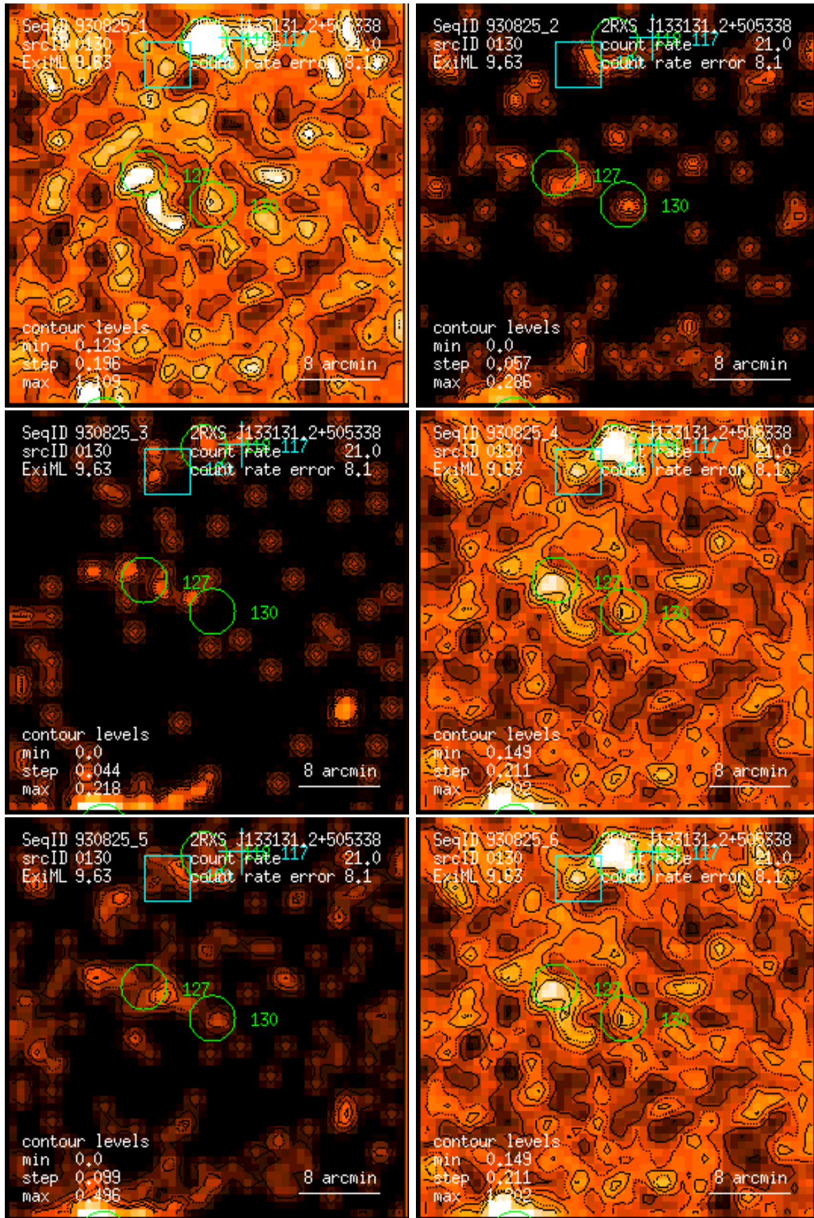
Figure 130: RASS 930825: detection 0130: band rate images, Gaussian filter: (1) PSPC channels 11 – 41, (2) 52 – 90, (3) 91 – 201, (4) 11 – 235, (5) 52 – 201, (6) 11 – 201. Broad band rates in counts/ks. Band rate contour levels in counts/ks/arcmin 2 .
