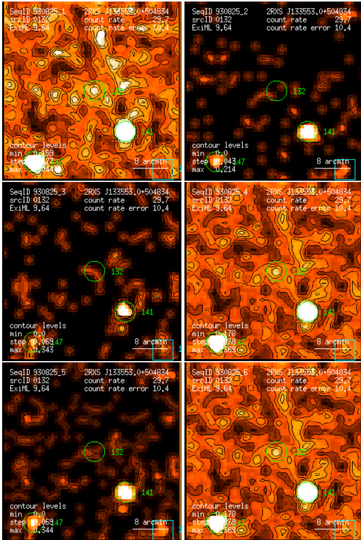
Figure 132: RASS 930825: detection 0132: band rate images, Gaussian filter: (1) PSPC channels 11 – 41, (2) 52 – 90, (3) 91 – 201, (4) 11 – 235, (5) 52 – 201, (6) 11 – 201. Broad band rates in counts/ks. Band rate contour levels in counts/ks/arcmin 2 .
