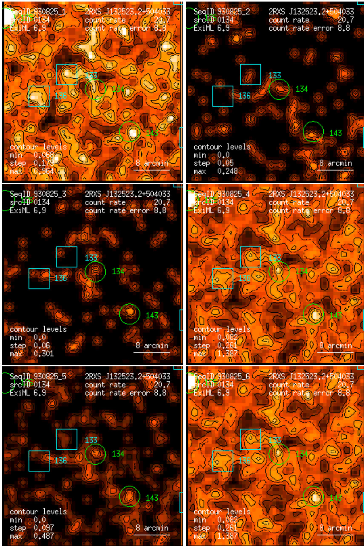
Figure 134: RASS 930825: detection 0134: band rate images, Gaussian filter: (1) PSPC channels 11 – 41, (2) 52 – 90, (3) 91 – 201, (4) 11 – 235, (5) 52 – 201, (6) 11 – 201. Broad band rates in counts/ks. Band rate contour levels in counts/ks/arcmin 2 .
