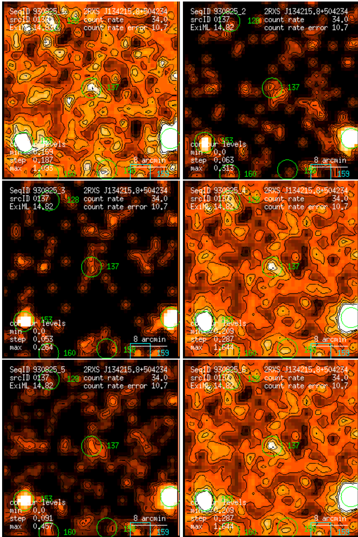
Figure 137: RASS 930825: detection 0137: band rate images, Gaussian filter: (1) PSPC channels 11 – 41, (2) 52 – 90, (3) 91 – 201, (4) 11 – 235, (5) 52 – 201, (6) 11 – 201. Broad band rates in counts/ks. Band rate contour levels in counts/ks/arcmin 2 .
