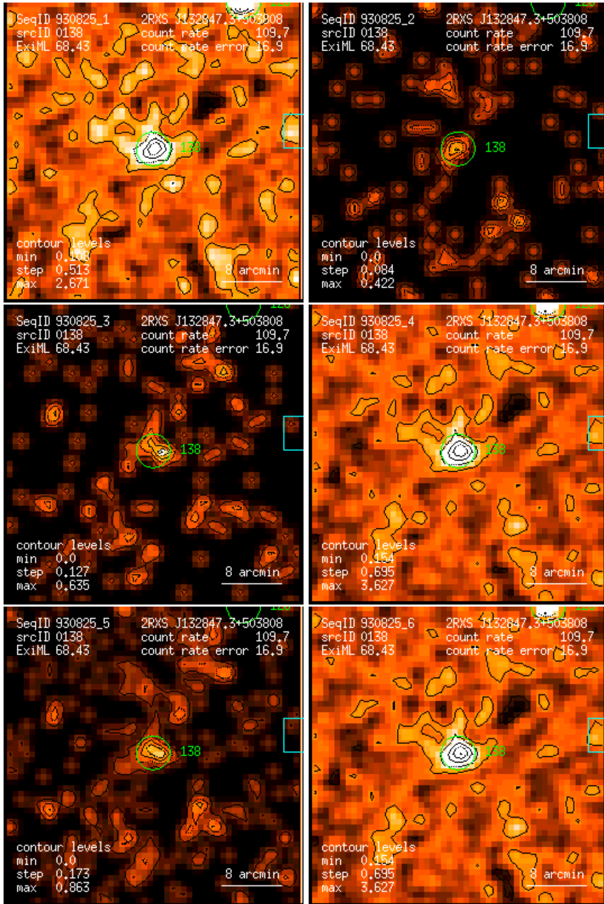
Figure 138: RASS 930825: detection 0138: band rate images, Gaussian filter: (1) PSPC channels 11 – 41, (2) 52 – 90, (3) 91 – 201, (4) 11 – 235, (5) 52 – 201, (6) 11 – 201. Broad band rates in counts/ks. Band rate contour levels in counts/ks/arcmin 2 .
