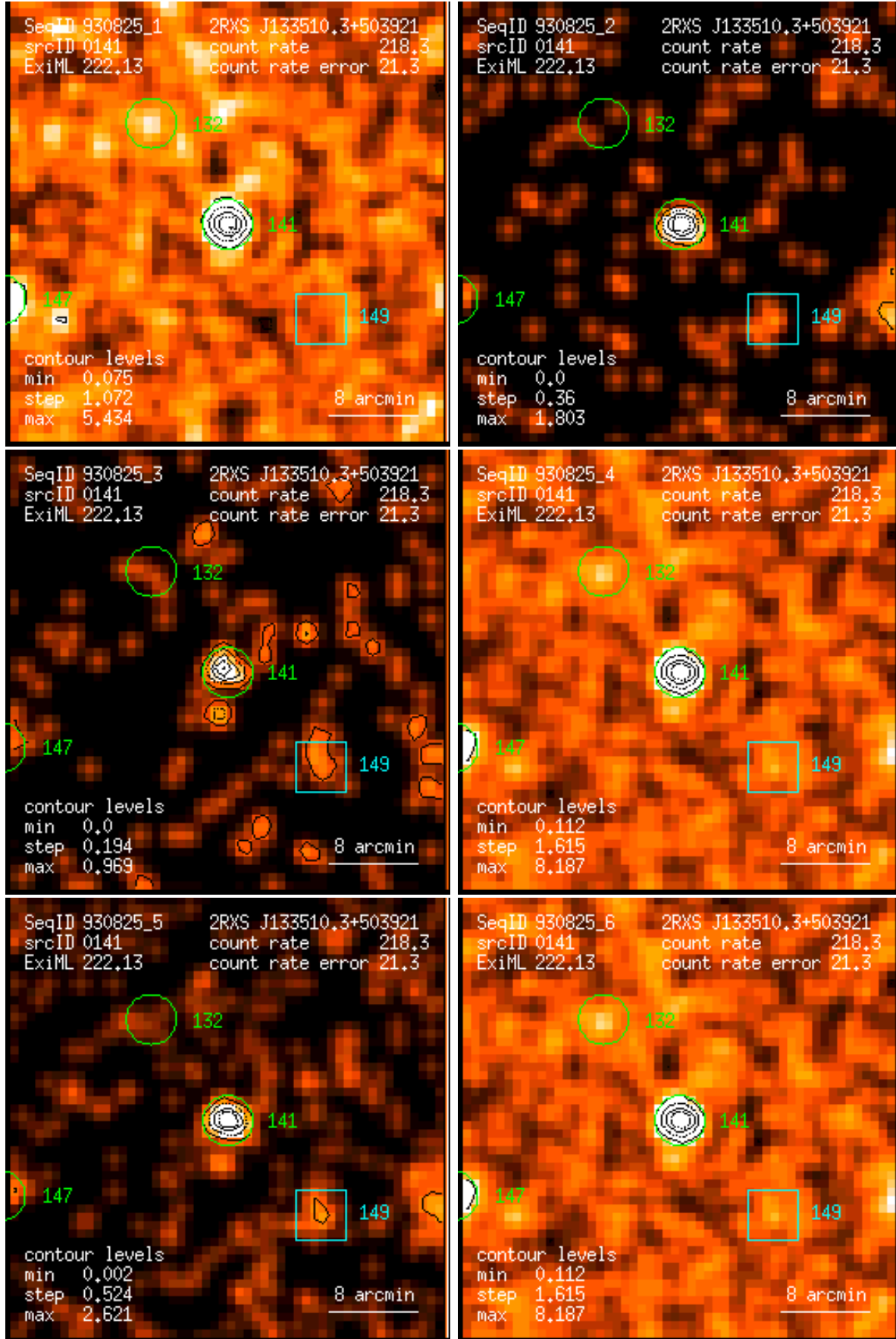
Figure 141: RASS 930825: detection 0141: band rate images, Gaussian filter: (1) PSPC channels 11 – 41, (2) 52 – 90, (3) 91 – 201, (4) 11 – 235, (5) 52 – 201, (6) 11 – 201. Broad band rates in counts/ks. Band rate contour levels in counts/ks/arcmin 2 .
