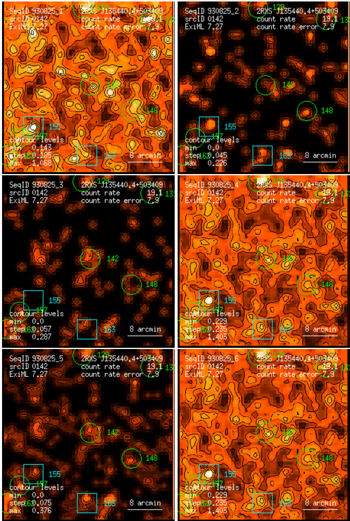
Figure 142: RASS 930825: detection 0142: band rate images, Gaussian filter: (1) PSPC channels 11 – 41, (2) 52 – 90, (3) 91 – 201, (4) 11 – 235, (5) 52 – 201, (6) 11 – 201. Broad band rates in counts/ks. Band rate contour levels in counts/ks/arcmin 2 .
