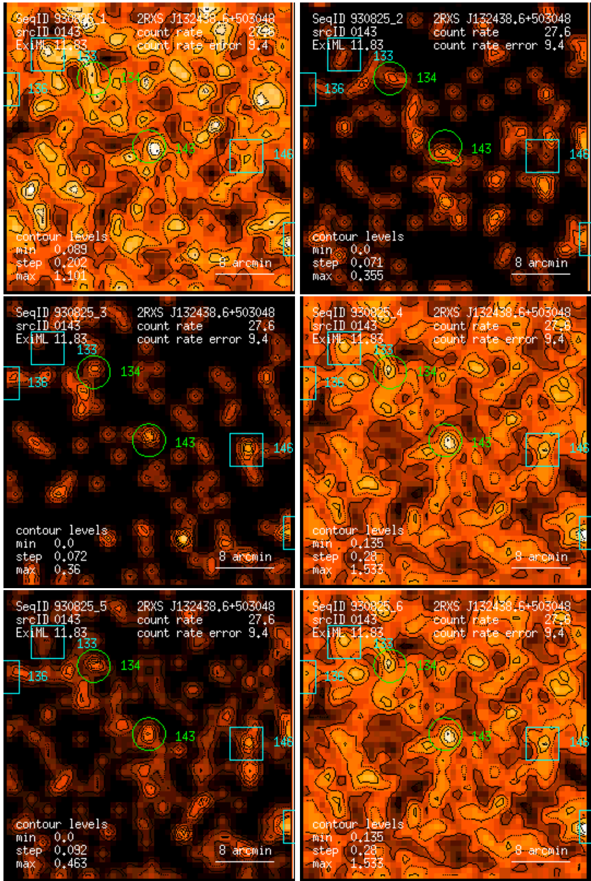
Figure 143: RASS 930825: detection 0143: band rate images, Gaussian filter: (1) PSPC channels 11 – 41, (2) 52 – 90, (3) 91 – 201, (4) 11 – 235, (5) 52 – 201, (6) 11 – 201. Broad band rates in counts/ks. Band rate contour levels in counts/ks/arcmin 2 .
