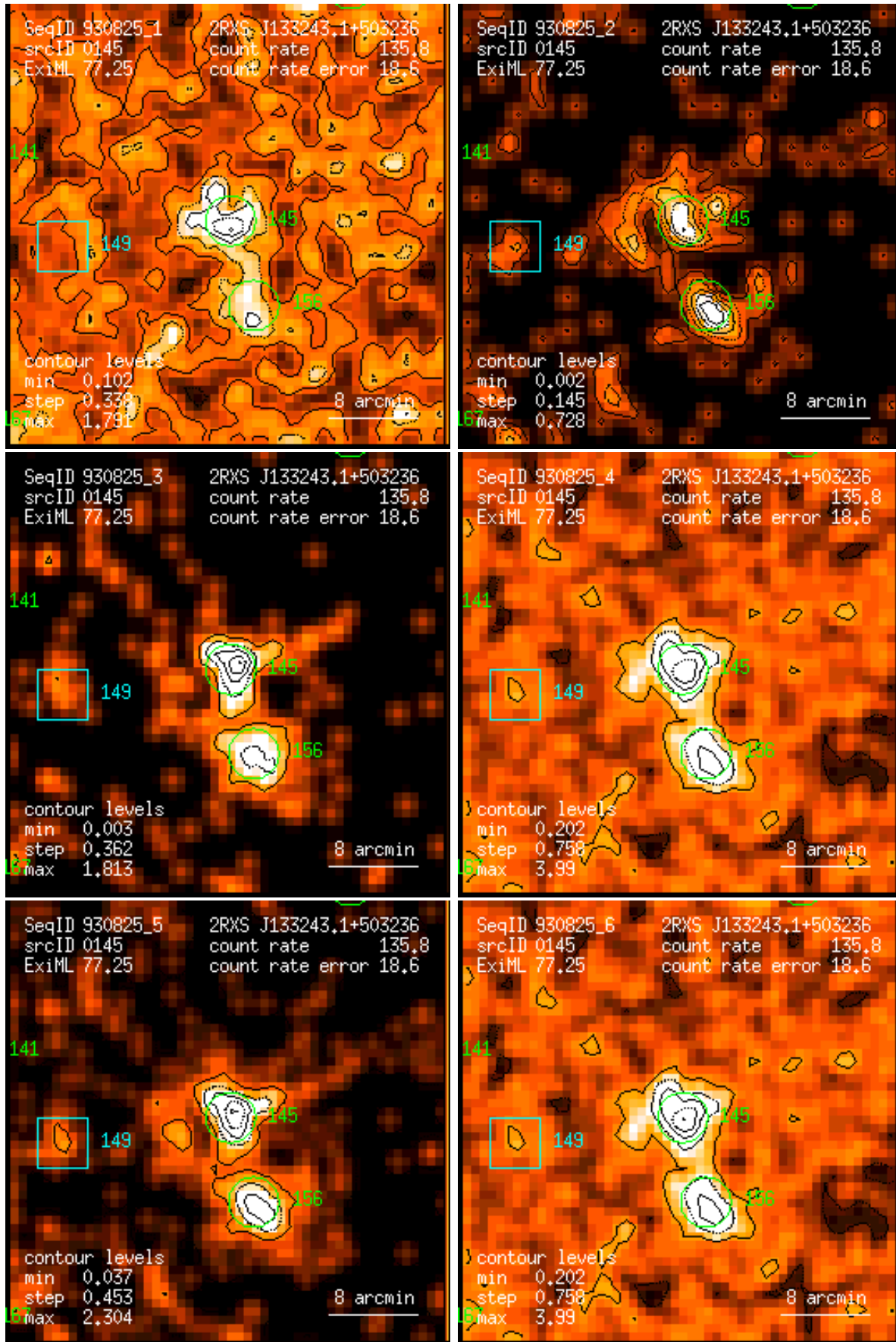
Figure 145: RASS 930825: detection 0145: band rate images, Gaussian filter: (1) PSPC channels 11 – 41, (2) 52 – 90, (3) 91 – 201, (4) 11 – 235, (5) 52 – 201, (6) 11 – 201. Broad band rates in counts/ks. Band rate contour levels in counts/ks/arcmin 2 .
