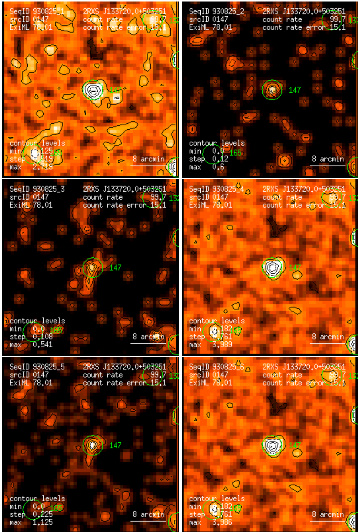
Figure 147: RASS 930825: detection 0147: band rate images, Gaussian filter: (1) PSPC channels 11 – 41, (2) 52 – 90, (3) 91 – 201, (4) 11 – 235, (5) 52 – 201, (6) 11 – 201. Broad band rates in counts/ks. Band rate contour levels in counts/ks/arcmin 2 .
