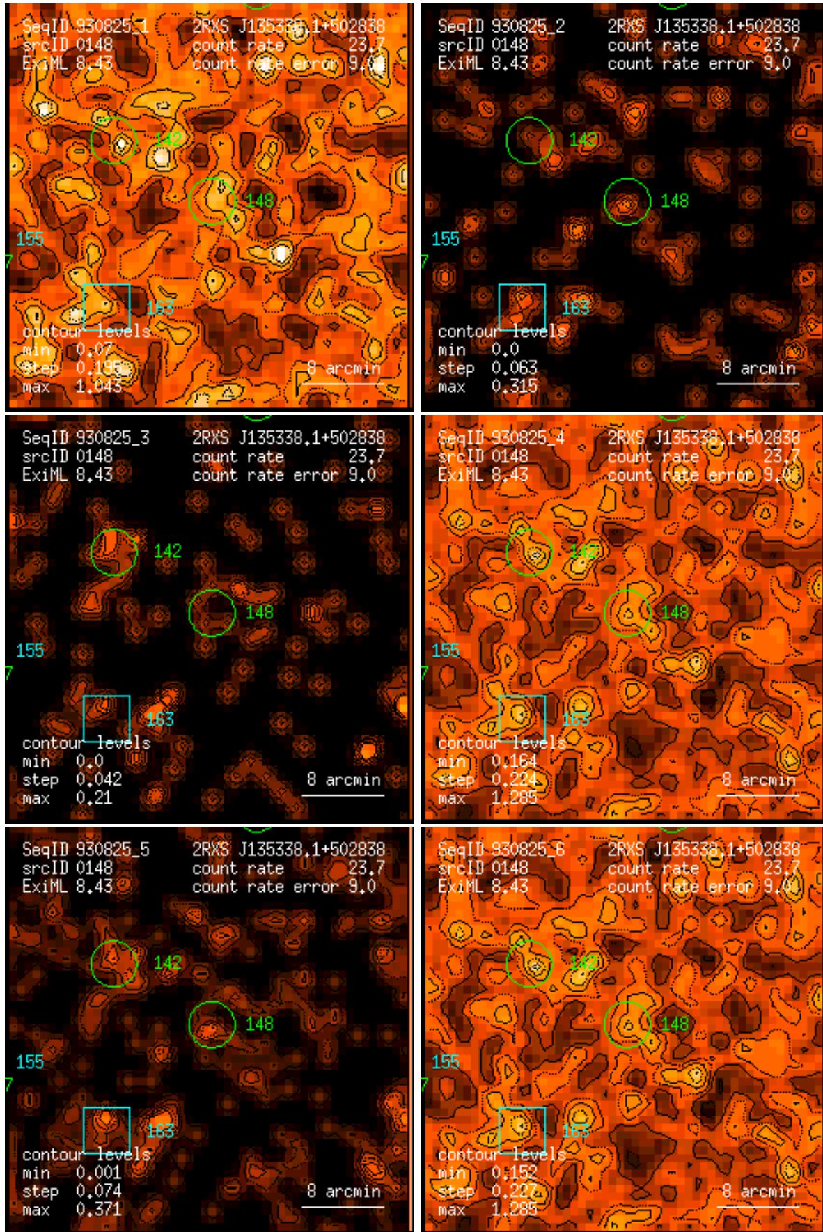
Figure 148: RASS 930825: detection 0148: band rate images, Gaussian filter: (1) PSPC channels 11 – 41, (2) 52 – 90, (3) 91 – 201, (4) 11 – 235, (5) 52 – 201, (6) 11 – 201. Broad band rates in counts/ks. Band rate contour levels in counts/ks/arcmin 2 .
