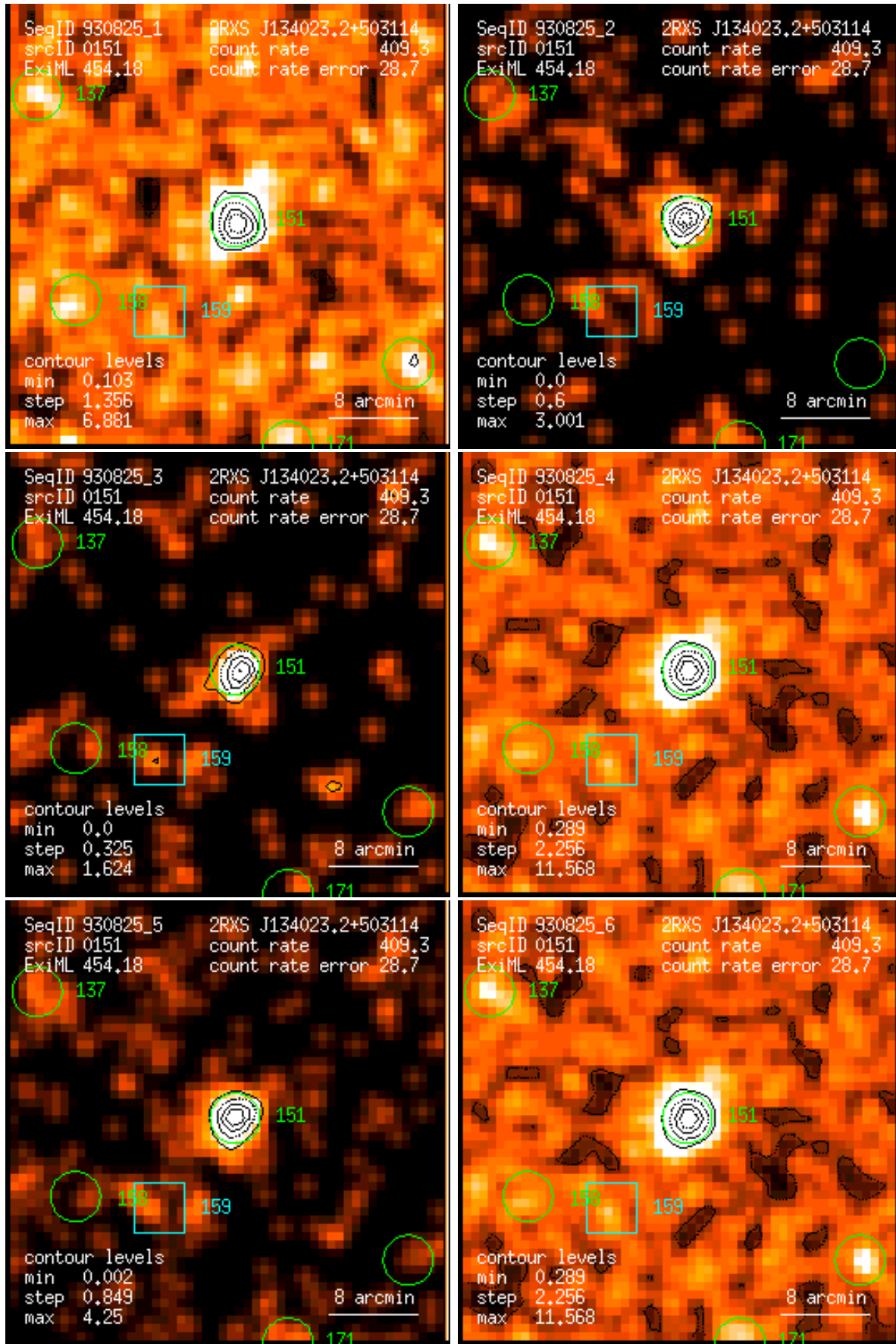
Figure 151: RASS 930825: detection 0151: band rate images, Gaussian filter: (1) PSPC channels 11 – 41, (2) 52 – 90, (3) 91 – 201, (4) 11 – 235, (5) 52 – 201, (6) 11 – 201. Broad band rates in counts/ks. Band rate contour levels in counts/ks/arcmin 2 .
