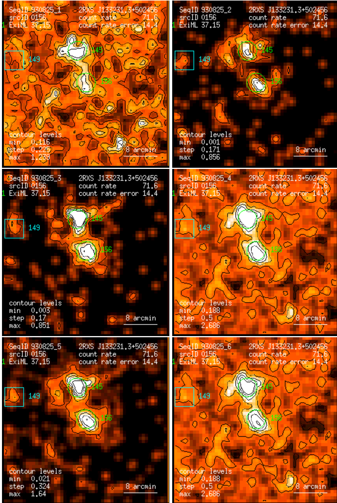
Figure 156: RASS 930825: detection 0156: band rate images, Gaussian filter: (1) PSPC channels 11 – 41, (2) 52 – 90, (3) 91 – 201, (4) 11 – 235, (5) 52 – 201, (6) 11 – 201. Broad band rates in counts/ks. Band rate contour levels in counts/ks/arcmin 2 .
