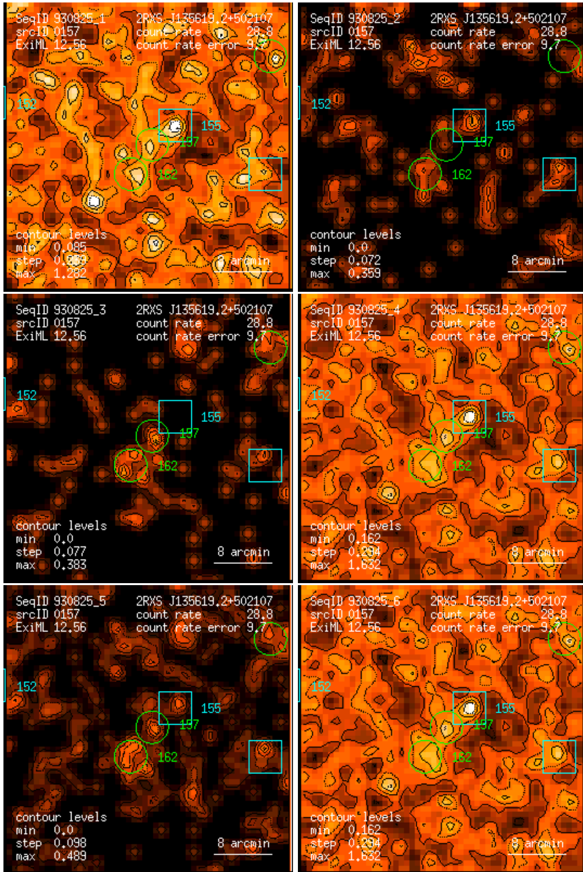
Figure 157: RASS 930825: detection 0157: band rate images, Gaussian filter: (1) PSPC channels 11 – 41, (2) 52 – 90, (3) 91 – 201, (4) 11 – 235, (5) 52 – 201, (6) 11 – 201. Broad band rates in counts/ks. Band rate contour levels in counts/ks/arcmin 2 .
